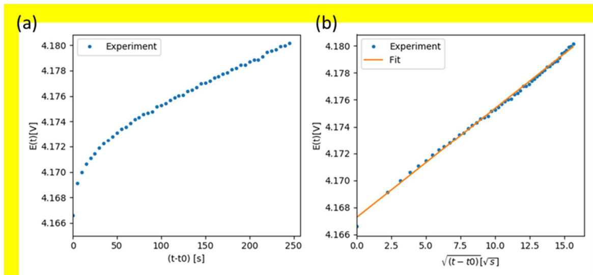
Fig. 4 : \text{Ni}_{0.6}\text{Mn}_{0.2}\text{Co}_{0.2}\text{O}_2 vs. Li GITT experiment (a) Cell voltage as a function of time during a charging current pulse (b) Cell voltage vs square root time for the same charging current pulse with the corresponding linear fit
