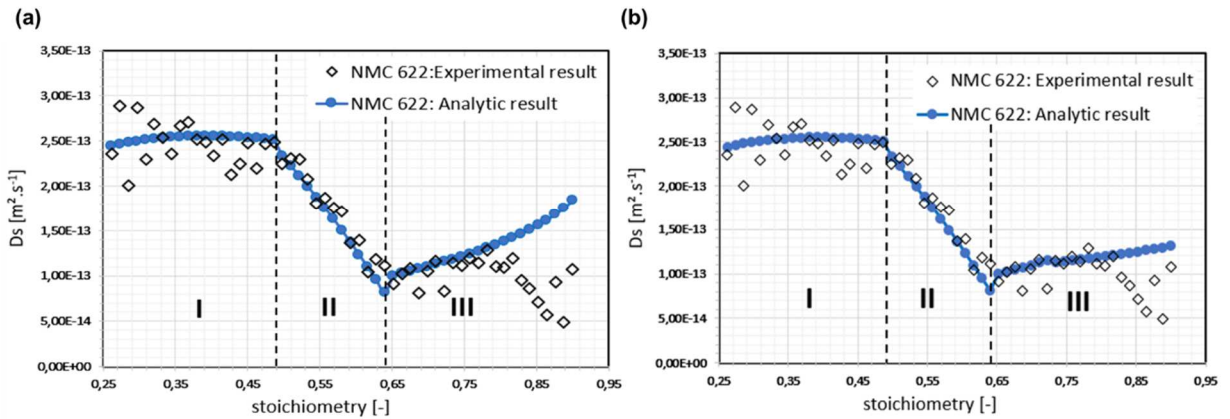
Fig. 11: Validation of the model equation of the Ni_{0.6}Mn_{0.2}Co_{0.2}O_2 D_s
