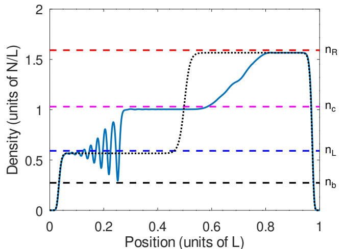
FIG. 7. (color online) Density profile in the box at time t = 1.5 \times 10^{-3} \times mL^2/\hbar (solid blue line) for a initial dam-break problem (dotted black line), with V_1 = 0 and V_{\text{offset}} = gN . The four horizontal dashed lines correspond to the analytical formula for n_R , n_c , n_L , n_b , respectively. The small discrepancy with the numerical solution may be attributed to finite size effects.
