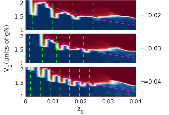
FIG. 8. Normalized power spectrum density at zero frequency as a function of central barrier height V_1 and initial imbalance z_0 for a quench of \tau = \{0.02, 0.03, 0.04\} (top, middle, bottom). The magenta dashed line indicates the prediction of the two-mode model for the self-trapping transition. The dashed vertical green lines correspond to the predicted resonances.
