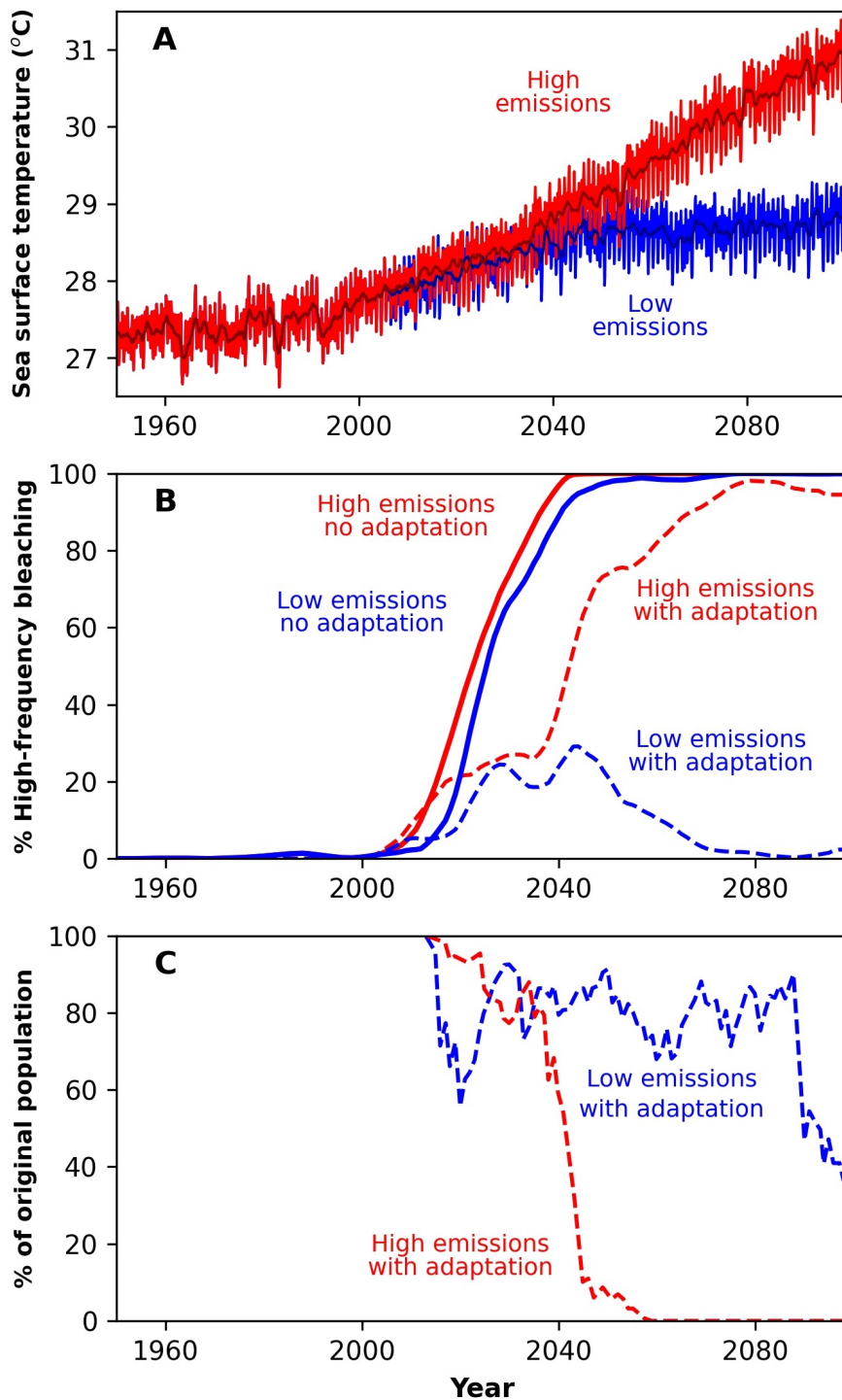
Figure 1. Modeled projections of average sea surface temperature and bleaching: (A) temperatures for high (RCP8.5) and low (RCP2.6) emissions scenarios, and (B) the percentage of 1x1 degree reef cells experiencing high-frequency bleaching ( \geq 2 severe events per decade) for four combinations of mitigation and adaptation; lines are smoothed with 10-year moving averages. For comparison, (C) is the change in modeled coral population size under a multi-locus genetic adaptation model at different future emission levels (Bay et al., 2017), beginning in year 2010. The dashed lines in (B) showing bleaching frequency with adaptation are mirrored by the lines in (C) showing percentage of original coral population size.
