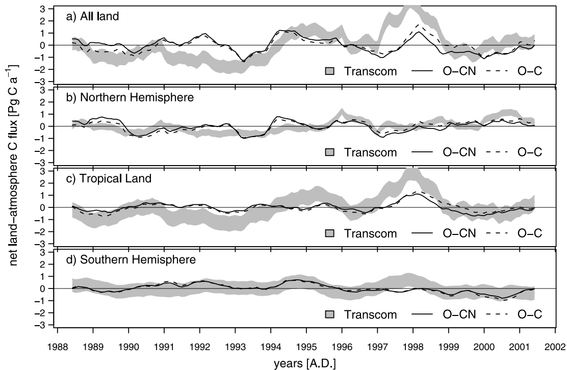
Figure 4. Interannual variability of the net land-atmosphere C exchanges (1988–2002) for (a) global, (b) northern extratropical, (c) tropical, and (d) southern extratropical land regions. The time series are 12 months running mean with the mean seasonal cycle removed. The gray area indicates the mean \pm standard deviation of the Transcom3 inversion study [Baker et al. , 2006]. The Transcom3 study used 13 atmospheric transport models, observed time series of atmospheric [\text{CO}_2] at 78 stations, and the average seasonal net terrestrial and ocean \text{CO}_2 fluxes as prior estimates, as well as a seasonal wind field.
