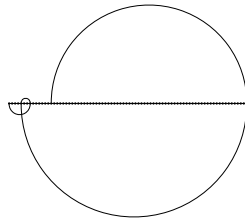
(a) n_1 = 80 is its supremum element.
