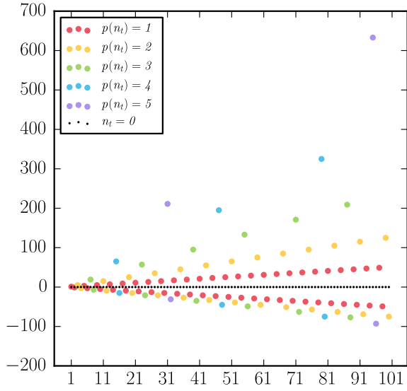
Figure 7: Subsequences 1 \leq p(n_t) \leq 5 of F contained within c(n_t) but now without the addition term n_t , or (n \equiv 1) d^l(n) (3^{p(n)} - 2^{p(n)}) - (n \equiv 0) d^l(n) (2^{p(n)} - 1) \pmod{2} .
