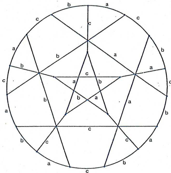
Fig. 1. A largest (3, 3)_C -graph, with a 3-coloring of its edges.
