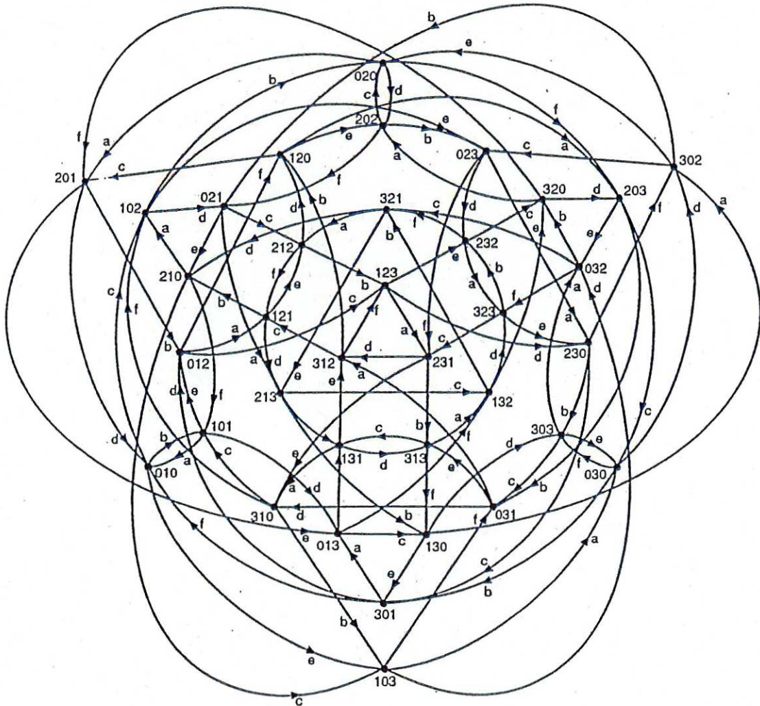
Fig. 2. The (6, 3)_C -digraph K(3, 3) , with a 6-coloring of the arcs.
