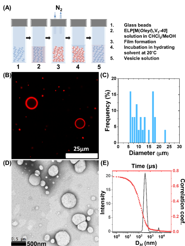
Figure 2. (A) Schematic representation of the glass beads thin film hydration process in water. (B) Confocal laser scanning microscopy image (red channel) of giant lipo-proteinosomes (GLPs) obtained using 5 mm beads) at room temperature, and (C) size distribution histogram plotted from the counting of 25 vesicles. (D) Uranyl acetate-stained TEM image of nanometer sized lipo-proteinosomes (NLPs) obtained using 0.5 mm beads) with an average size of 295±62 nm ( n=20 ) and (E) 90° angle DLS intensity-averaged distribution of
