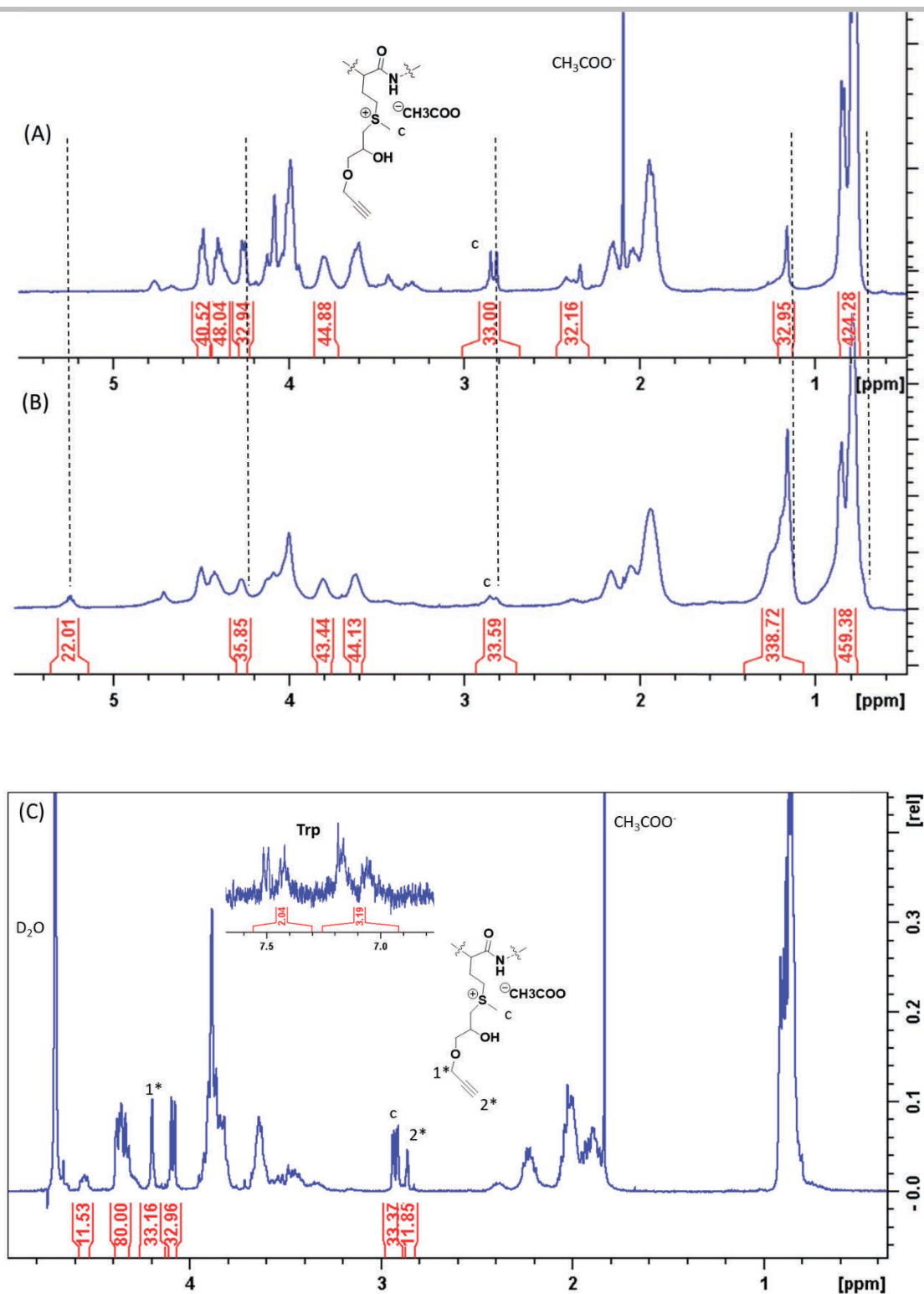
Figure S4. ^1\text{H} NMR spectrum of (A) ELP[M( Alkyne ) 1 V 3 -40] and (B) ELP[M( Oleyl ) 1 V 3 -40] in \text{CDCl}_3 (15% TFA-d) and (C) ELP[M( Alkyne ) 1 V 3 -40] (data provided only serve for comparison with the new product claimed) [3],[4] in \text{D}_2\text{O} at room temperature.
