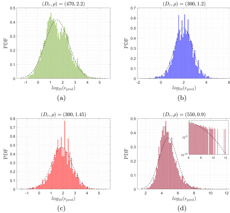
Figure 5: The error in logarithmic scale in the prediction phase, calculated at t_{\text{pred}} = 25 , of an incremented set of N = 5000 realisations is shown in histogram plots for four different RC configurations. The distribution is binned in n_{\text{bins}} = 100 samples. The black dashed curves represent the unimodal normal PDF, whose mean value and standard deviation are the mean value and the standard deviation of the error distribution functions for the corresponding configuration.
