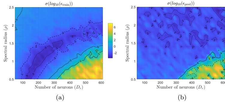
Figure 3: The standard deviation \sigma of the logarithm in base 10 of the errors, for both training (a) and prediction (b) phases, within the set of N = 500 realisations is displayed for the same scans reported in figure 2. The large variation within the whole set of realisations can be thus appreciated.
