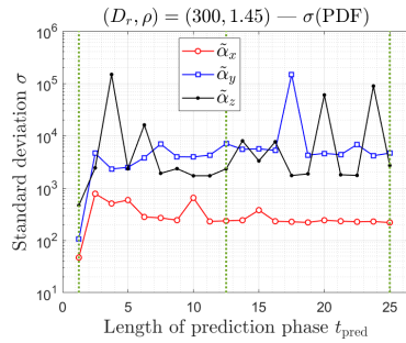
Figure 10: The evolution in time of the standard deviation \sigma of the \alpha coefficient PDFs displayed in figure 9 is shown in logarithmic scale for the prediction phase up to t_{\text{pred}} = 25 . The green dashed vertical lines represent the time windows displayed in figure 9.
