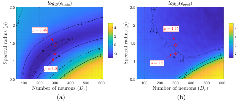
Figure 2: A scan of the error 13, in logarithmic scale, over the input parameters D_r and \rho of the reservoir network is displayed for the training and the prediction phase, in panel (a) and (b) respectively. The errors are averaged over the whole set of realisations ( N = 500 ) for each couple (D_r, \rho) . Highlighted with red markers are the configuration employed in Ref. [18].
