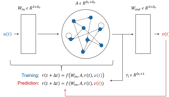
Figure 1: Schematic representation of the reservoir computing paradigm.
