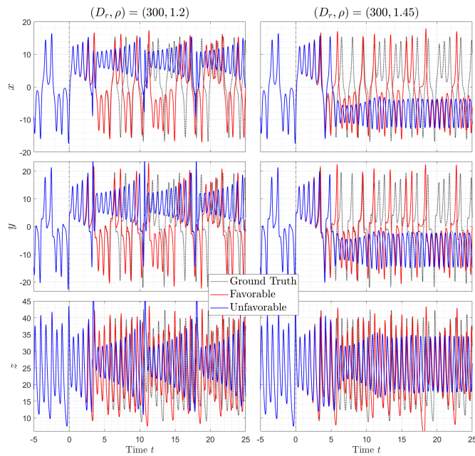
Figure 4: The dynamics of the three components of the Lorenz system, predicted by the RC, is shown for the two configurations studied in Ref. [18], i.e. (D_r, \rho) = (300, 1.2) (left column) and (D_r, \rho) = (300, 1.45) (right column). The black dotted curves are the actual chaotic trajectories obtained through numerical integration of the Lorenz equations with the RK4 method (labelled as Ground truth in the legend). Red and blue curves show respectively the best and a non-favorable solution obtained through RC technique over the whole set of N = 500 realisations.
