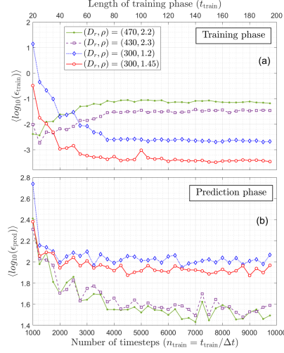
Figure 7: The errors in the training (a) and in the prediction phase (b) are shown as a function of the length of the training phase for four different input configurations of the reservoir network. The configurations are the same analyzed also in figures 5 and 6. The abscissas is expressed both in length of the training phase in normalized time t_{\text{train}} and in number of time steps n_{\text{train}} in the training phase.
