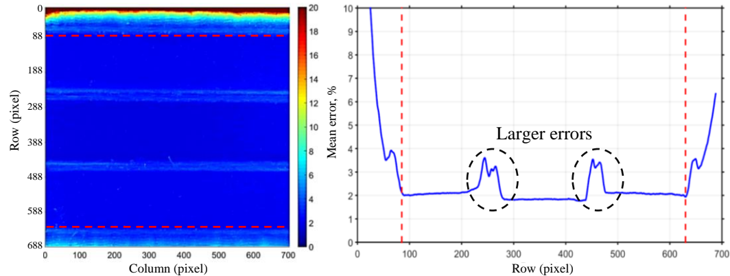
FIG. 29. Mean measurement error of vapor volume fraction estimated from pure air images.
