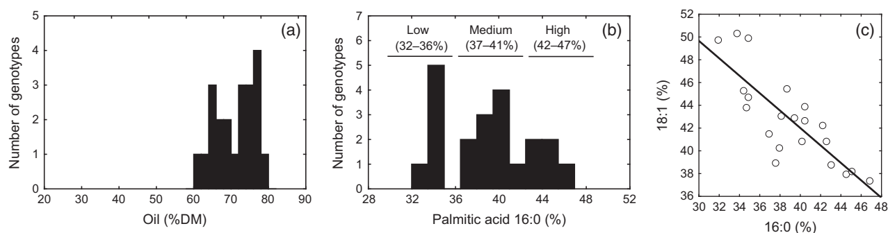
Figure 1. Distribution of mesocarp oil content and 16:0 percentage in the backcrossed hybrid (BC) population
