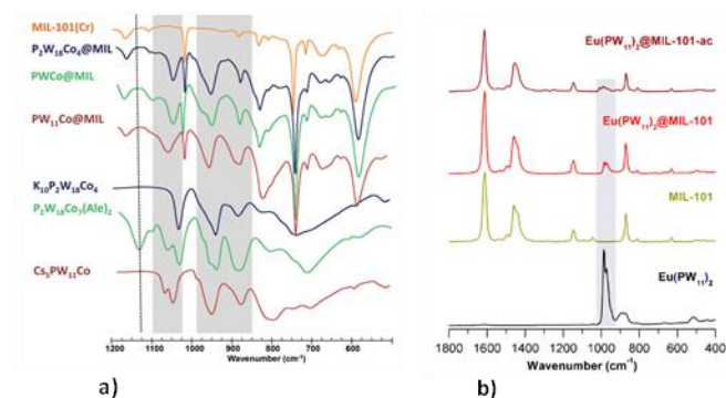
Fig. 10 a) IR spectra of composites synthesised by immobilising Co-substituted POMs in \text{MIL-101}(\text{Cr}) ; the composite named \text{PWCo}@\text{MIL} results from the immobilisation of the hybrid \text{P}_2\text{W}_{18}\text{Co}_7(\text{Ale})_2 POM. b) Raman spectra of \text{Eu}(\text{PW}_{11})_2@\text{MIL-101}(\text{Cr}) before ( \text{Eu}(\text{PW}_{11})_2@\text{MIL-101} ) and after ( \text{Eu}(\text{PW}_{11})_2@\text{MIL-101-ac} ) catalysis compared to that of the POM and MOF precursors. Reprinted from refs. 38 with permission from RSC and 64 (Copyright 2013 Elsevier B.V.) respectively.
