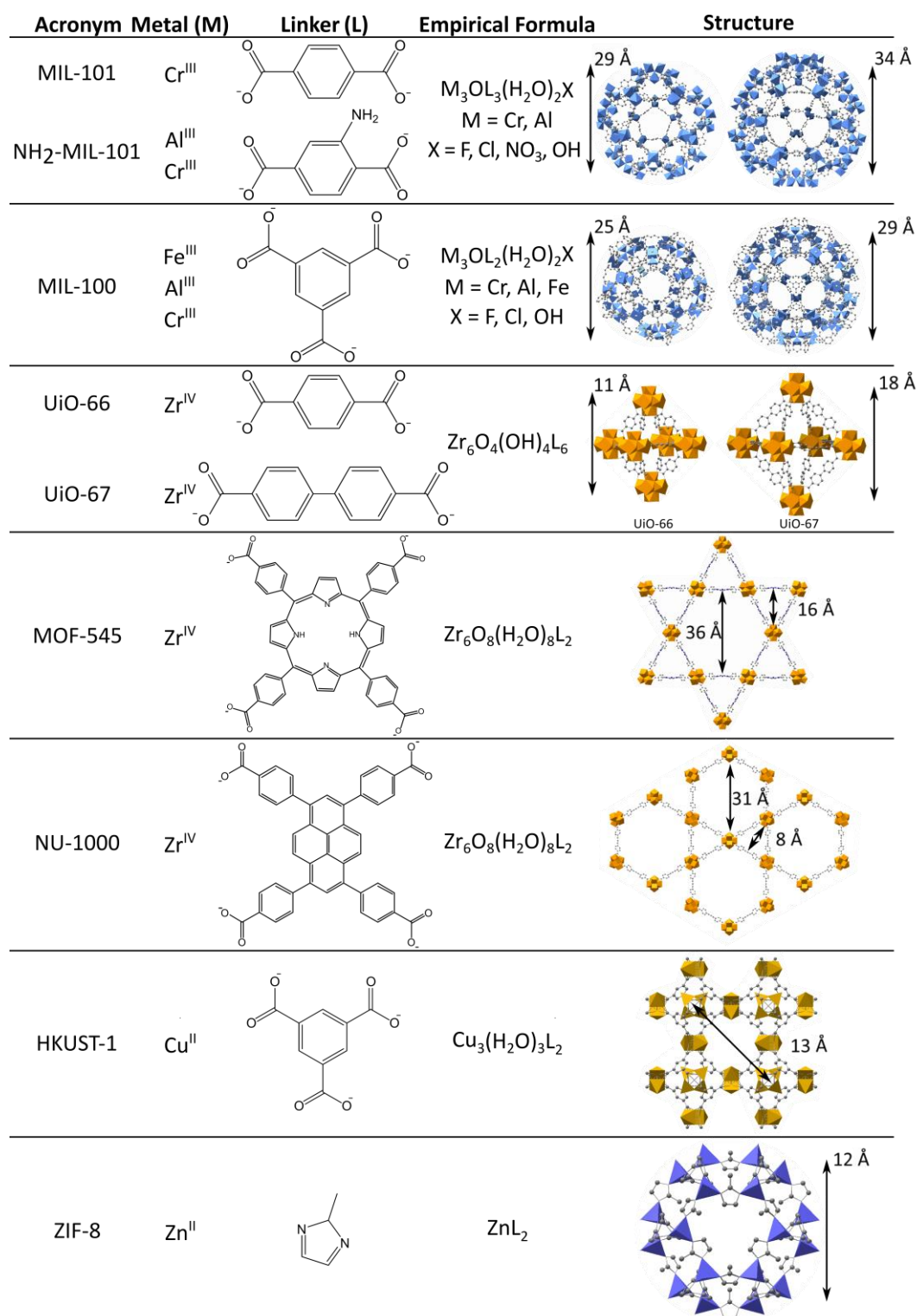
Fig. 1 Representation of the structures of the main MOF hosts reported in this review with the dimensions of the cavities, the linker's and MOF's formulas.
