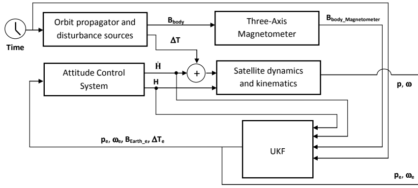
Fig. 1 Simulation scheme
