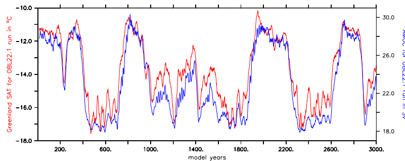
Fig. 9. Red: SAT over Greenland in °C for OBL22.1 run. SAT was averaged over 60° W to 30° W and 60° N to 80° N. Blue: AMOC for OBL22.1 run in Sv. A running mean of 25 years was applied for both timeseries.
