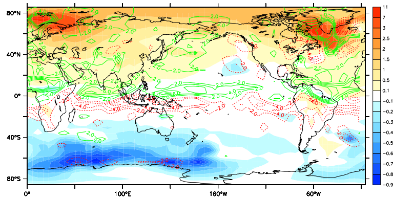
Fig. 8. SAT difference in K (shaded) and precipitation difference in cm/yr (contours) between a strong and a weak AMOC state for the OBL22.1 run. A weak (strong) state is defined by an AMOC <21 Sv (>27 Sv). See also Fig. 2i. Note the non-linear color scale for SAT difference.
