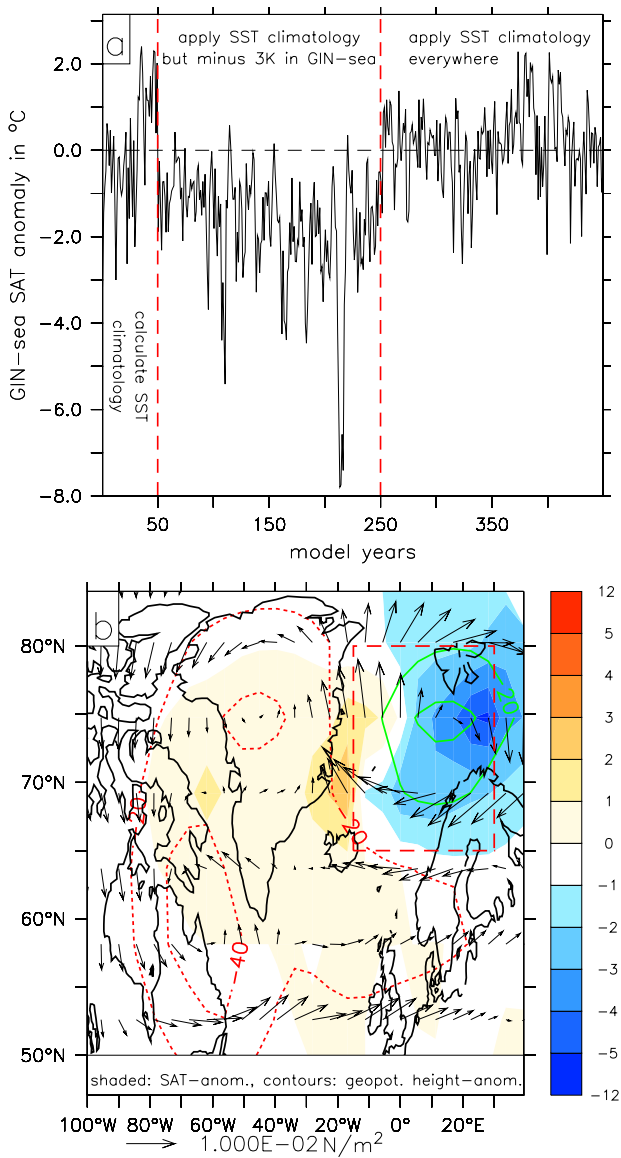
Fig. 5. (a) GIN Sea SAT anomaly (averaged over 15^{\circ} W to 30^{\circ} E and 65^{\circ} N to 80^{\circ} N) with respect to the model years 1 to 50 of the sensitivity experiment. The red lines separate the three stages of the experiment. (b) Anomalies in SAT in K (shaded), 800 mbar geopotential height in \text{m}^2/\text{s}^2 (contours) and wind stress (arrows) with respect to the model years 1 to 50 of the sensitivity experiment. The red rectangular indicates the region where the SST perturbation is applied to the GIN Sea atmosphere. Please refer to Sect. 4.3 for details.
