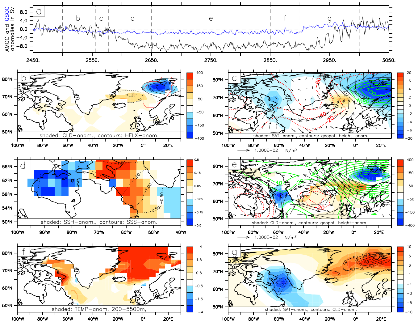
Fig. 3. (a) Anomalies of AMOC (black) and GSOAC (blue) in Sv for the OBL22.4 run for the timeframe 2450–3050 (see also Fig. 2c,h). Dashed vertical lines denote averaging intervals for panels b–g of this figure. (b) Anomalies in convective layer depth (CLD) in m (shaded) and surface heat flux (HFLX) in W/m 2 (contours). A positive HFLX anomaly is associated with a lower-than-normal heat loss of the surface ocean to the atmosphere. The red line indicates the mean GIN Sea sinking region in the model. (c) Anomalies of surface air temperature (SAT) in K (shaded), 800 mbar geopotential height in m 2 /s 2 (contours) and surface wind stress in N/m 2 (arrows). (d) Anomalies of sea surface height in m (shaded) and sea surface salinity in psu (contours). (e) Anomalies in CLD in m (shaded), 800 mbar geopotential height in m 2 /s 2 (contours) and surface wind stress in N/m 2 (arrows). (f) Anomalies of oceanic temperature in K averaged over 200–5500 m. (g) SAT anomalies in K (shaded) and CLD anomalies in m (contours). All anomalies in panels b–g are calculated against a strong AMOC state (years: 2400–2450) and averaged over the interval indicated by the respective letter in panel a.
