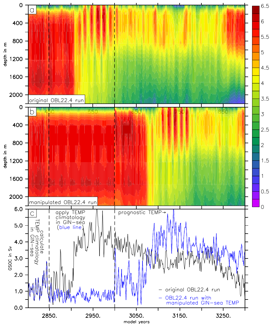
Fig. 7. Hovmoeller diagrams of temperature averaged over GIN Sea in ^{\circ}\text{C} for original OBL22.4 run (a) and (b) a restart of OBL22.4 run in which a subsurface temperature “climatology” in the GIN Sea was generated from the years 2801 to 2850 and prescribed for years 2851 to 3000. Subsequently the model were run another 300 years with prognostic temperatures in the GIN Sea. (c) GSOc for original (black line) and manipulated (blue line) OBL22.4 run in Sv for timeframe 2801–3300. Please refer to Sect. 4.3 for details.
