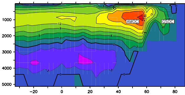
Fig. 1. Mean Atlantic Meridional Overturning Circulation for the control simulation in Sv. The two cells that are referred to in the text – GIN Sea overturning circulation (GSOC) and maximum of Atlantic overturning circulation (AMOC) – are indicated by the labels.
