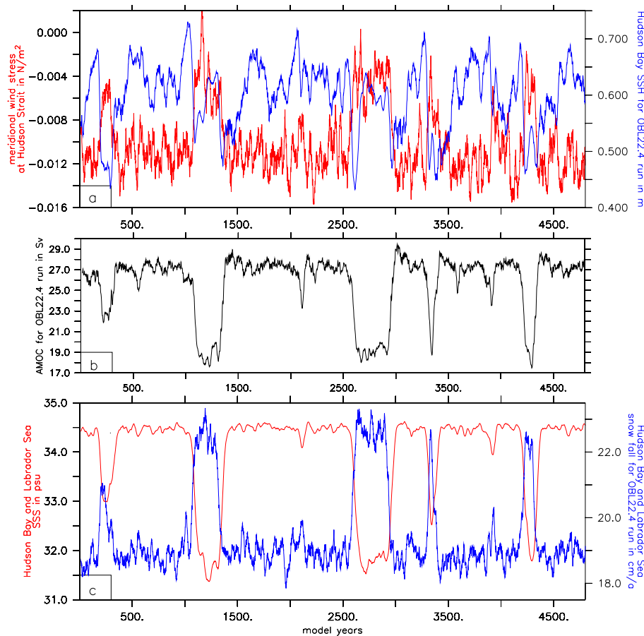
Fig. 4. Timeseries of variables for OBL22.4 run: (a) meridional wind stress at Hudson Strait ( 80^{\circ} W: 70^{\circ} W, 60^{\circ} N: 70^{\circ} N) (red) in \text{N/m}^2 and Hudson Bay ( 100^{\circ} W: 75^{\circ} W, 52^{\circ} N: 70^{\circ} N) sea surface height in m (blue) for OBL22.4 run. (b) AMOC in Sv for OBL22.4 run for comparison. (c) SSS in psu (red) and snow fall in \text{cm/a} (blue) averaged over Hudson Bay and Labrador Sea ( 100^{\circ} W: 45^{\circ} W, 50^{\circ} N: 70^{\circ} N) for OBL22.4 run in Sv. A running mean of 25 years was applied for all timeseries.
