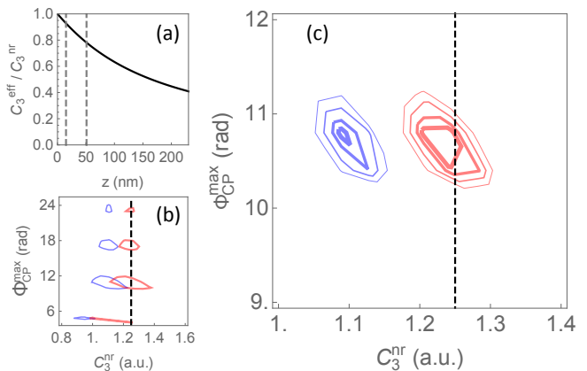
FIG. 3. (a): C_3^{\text{eff}}/C_3^{\text{nr}} as function of atom-surface distance. The two dashed lines represent the recorded atom-surface distance range. (b),(c): \chi_{\text{min}}^2 + n\sigma [ n=40 (b), n=1, 3, 6, 9 (c)] as functions of C_3^{\text{nr}} and \Phi_{\text{CP}}^{\text{max}} at 26.2 \text{ ms}^{-1} for vdW (blue) and CP (red) potentials. The dashed line shows the theoretical value for C_3^{\text{nr}} .
