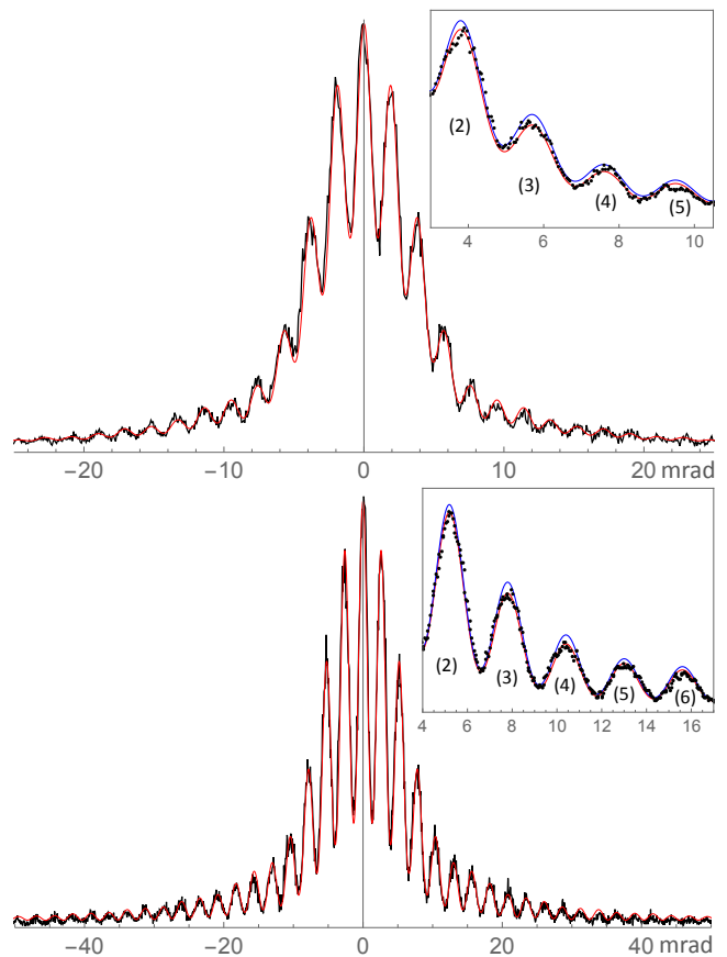
FIG. 2. Experimental diffraction spectra for beam velocities of 26 \text{ms}^{-1} (top) and 19.1 \text{ms}^{-1} (bottom) in black. The red curves are theoretical spectra with a single adjustable parameter ( d_0 ). The insets show individual diffraction orders. Black dots result from experimental spectra averaged over positive and negative diffraction orders. Red (blue) curves are calculated with CP (vdW) potentials.
