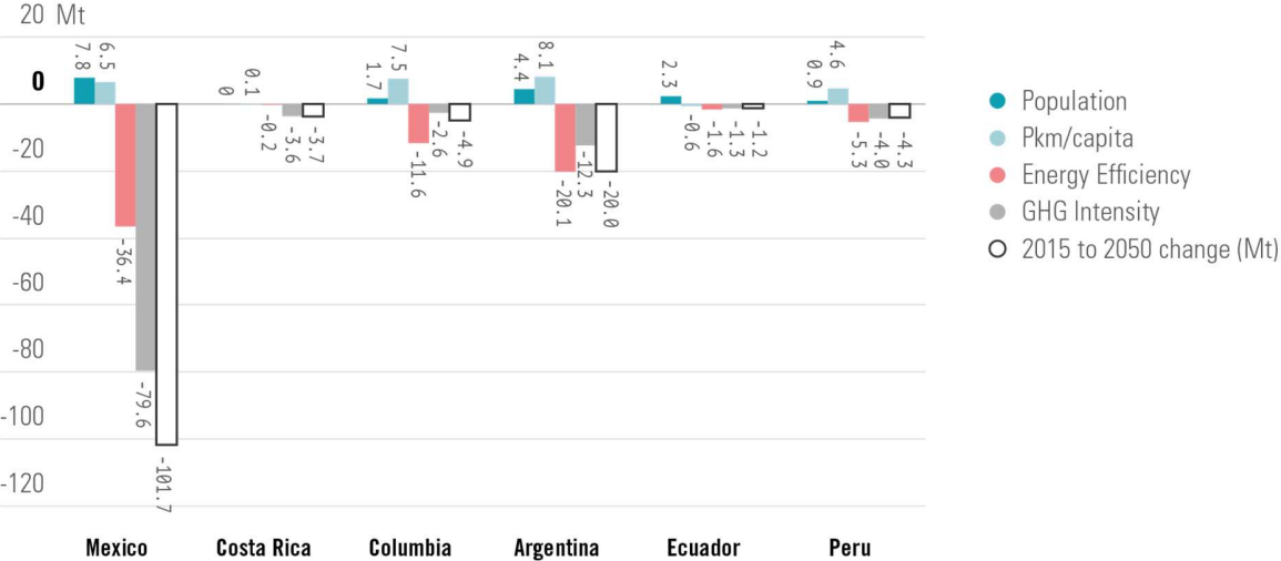
Figure 6 Changes in tonnes Mt CO 2 per year in 2050 compared to 2015 in passenger transport emissions due to population, pkm/capita, energy efficiency and end-use fuel GHG intensity
