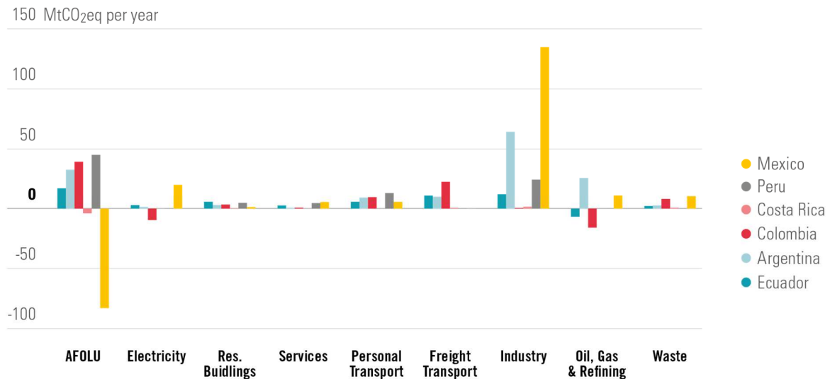
Figure 16 Remaining 2050 GHG emissions in the country DDPs, including negative fluxes (Mt/yr)
