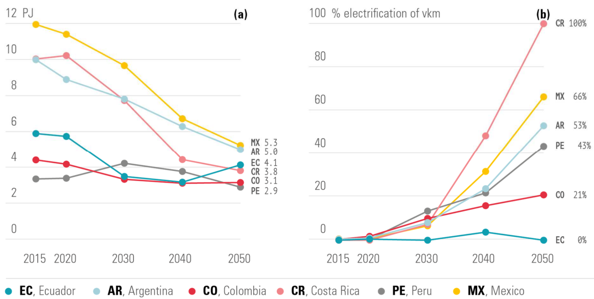
Figure 8 Total energy consumption for passenger transport (PJ) (a) and electrification of bus vkm (%) over time (MJ/pkm, 2015=1) (b).
