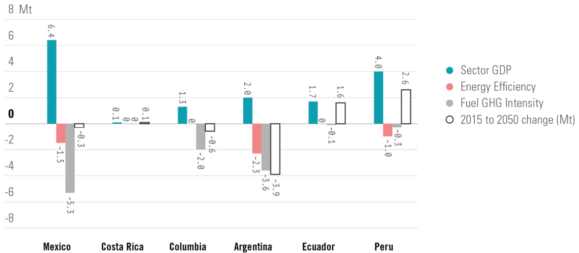
Figure 11 Changes in tonnes Mt CO 2 per year in 2050 compared to 2015 in the services sector due to GDP, energy efficiency and GHG intensity
