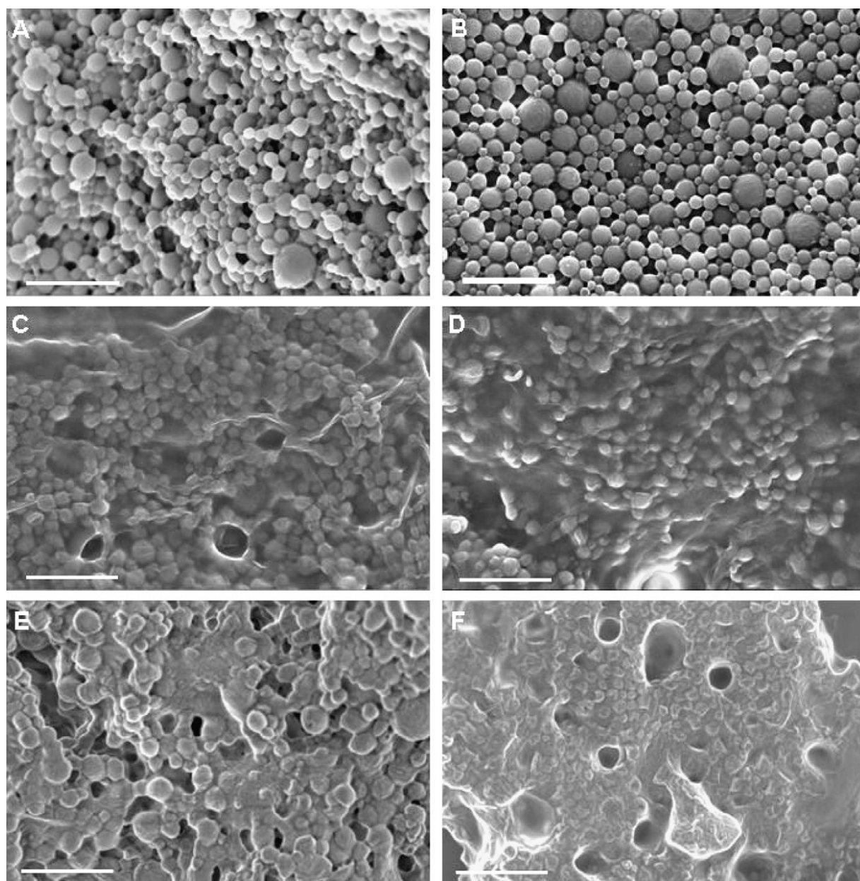
Figure 4. Scanning electron micrographs of the nanoparticle suspensions before (A), (C), (E) and after concentration (B), (D), (F) by dialysis of 3 g of the nanoparticle suspension against 5 mL of a solution of dextran 100,000 at a concentration of 300 g/L. (A and B) PIBCA-NS purif . (C and D) PCL-NS. (E and F) PCL-NC.
