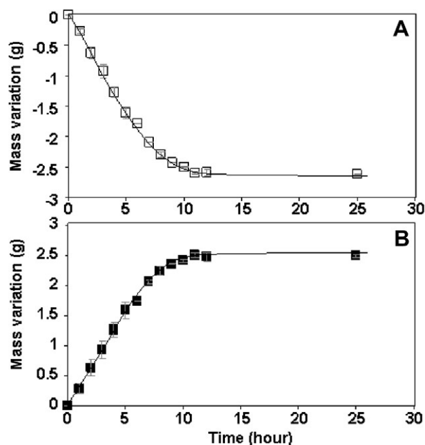
Figure 1. Kinetics of weight loss from the dialysis bag (A) and of weight gain in the counter-dialysis medium (B) during an experiment where 3 g of a PIBCA-NS purif suspension was dialyzed against 5 mL of counter-dialyzing solution containing 300 g/L of dextran 100,000.
