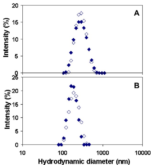
Figure 7. Size distributions obtained from photocorrelation spectroscopy measurements of the nanoparticle dispersions. Open symbols: parent nanoparticle suspension. Closed symbols: concentrated nanoparticle suspension. (A) PCL-NC purif . (B) PCL-NS purif .
