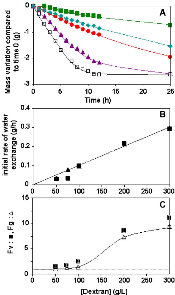
Figure 2. Effect of the concentration of dextran 100,000 in the counter dialyzing solution on the concentration of the nanoparticle suspension of PIBCA-NS purify . The amount of the nanoparticle sample was 3 g in all the experiments. (A) Kinetic of the weight loss of the dialysis bag: (A) Kinetics of the weight loss of the dialysis bag: effect (green square) 50 g/L, (blue diamond) 75 g/L, (red circle) 100 g/L, (purple triangle) 200 g/L, (h) 300 g/L. Dialysis experiments were performed with 5 mL of the counter-dialyzing medium. (B) Rate of water exchange calculated from the weight loss of the dialysis bag (black triangle) and from the weight gain of the counter-dialyzing medium (Black square). (C) Concentration factors.
