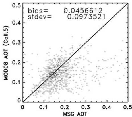
Figure 13. Scatterplot of SEVIRI and MODIS (Collection 5) monthly AOT values averaged over 1^\circ \times 1^\circ boxes on the MSG disk from June 2006 to September 2006 at 0.65 \mu\text{m} . Only SEVIRI AOT retrievals with a high degree of confidence (see text) and the corresponding MODIS AOT are considered.
