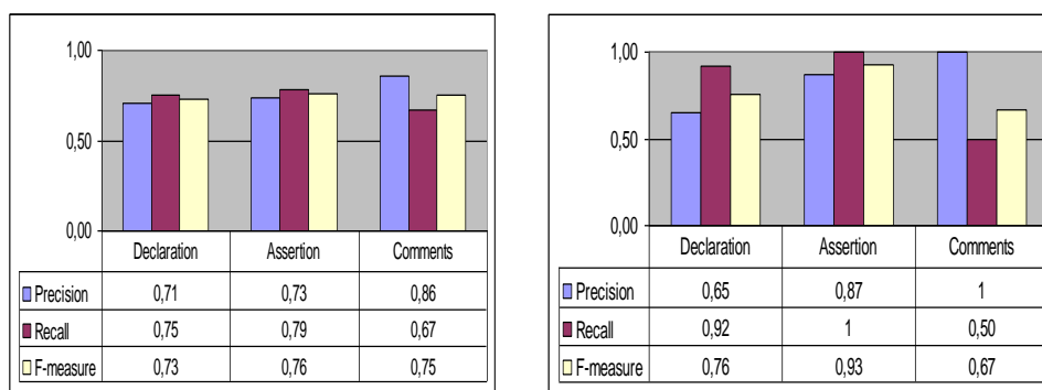
Fig.3. The results of evaluation on the Arabic (left) and French (right) corpora
