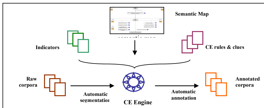
Fig.2. Simplified architecture of the platform EXCOM
