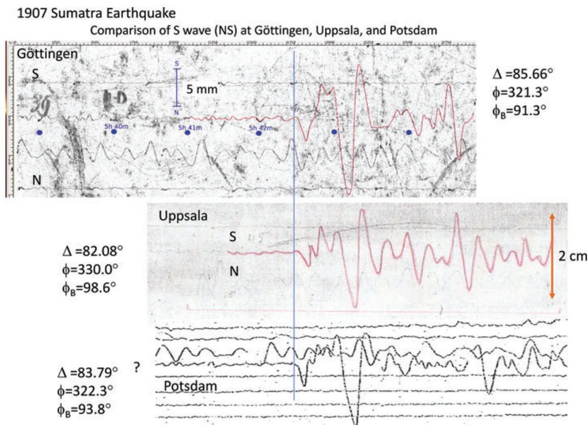
Figure 12. Comparison of the S wave on the NS component seismograms at Göttingen and Uppsala. Note the similarity of the waveform, and the northward first motion. The Potsdam seismogram is shown just for comparison.
