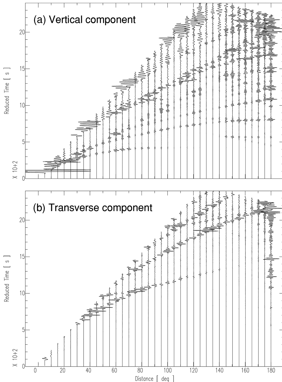
Figure 2. Epicentral distance plots for an earthquake at the central Mid-Atlantic Ridge ( M_w 6.2; event 8 in Table 1). The synthetic seismograms depict ground velocity and were computed using SPECFEM3D_GLOBE (Komatitsch & Tromp 2002a,b) for the 3-D mantle circulation model S09-M2-Q. The traces have been low-pass filtered at 0.09 Hz to remove numerical noise below 10 s period. Surface wave energy has been removed for better visualization of body wave phases and traces have been shifted along the time axis with a dynamic delay given by 0.04\Delta s. The dissipation of seismic energy due to intrinsic anelasticity has not been taken into account in the simulation.
