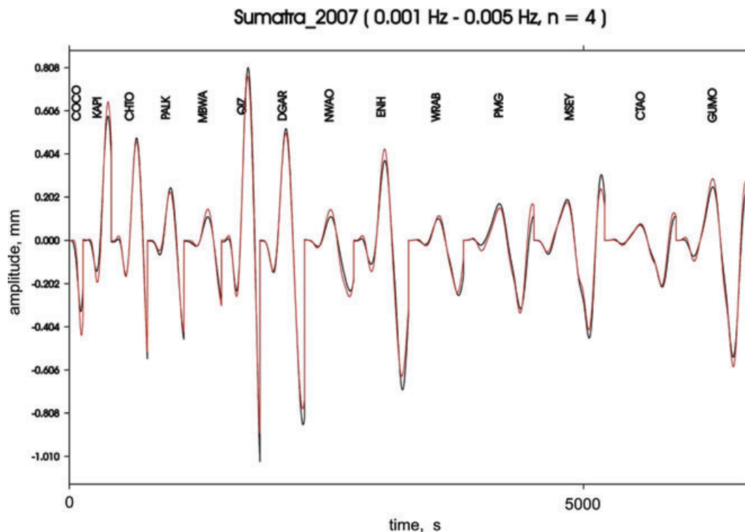
Figure 8. Concatenated observed (black trace) and synthetic (red trace) W phase. The window length (in s) is \Delta(\text{in degree})/n \text{ min} . In this case n = 4 .
