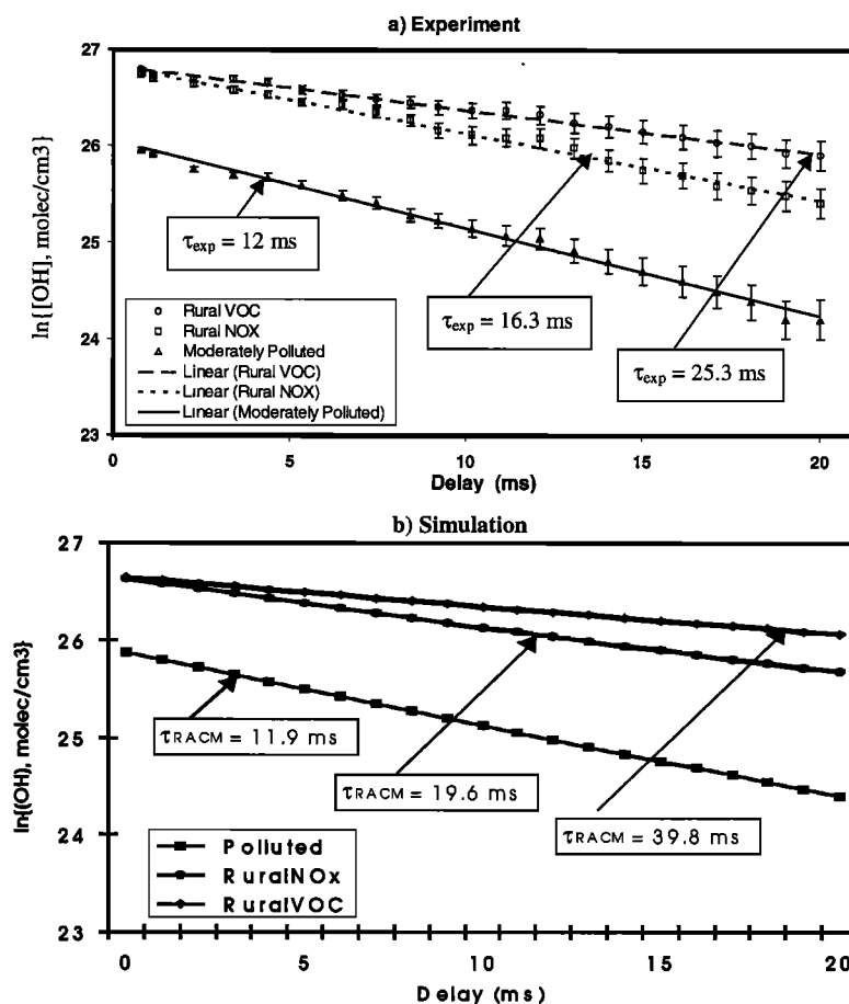
Figure 6. Natural logarithm of the pump and probe OH concentration versus time measured in the reaction cell for the three different NO x /VOC/O 3 gas mixtures defined in Table 2: (a) experimental values and (b) RACM-predicted results. OH lifetimes \tau are given by the slope of the linear fits. The experimental error bars represent the overall uncertainty of the statistical variability of the fluorescence signal and variations in the trace gas concentrations, assumed to be random.
