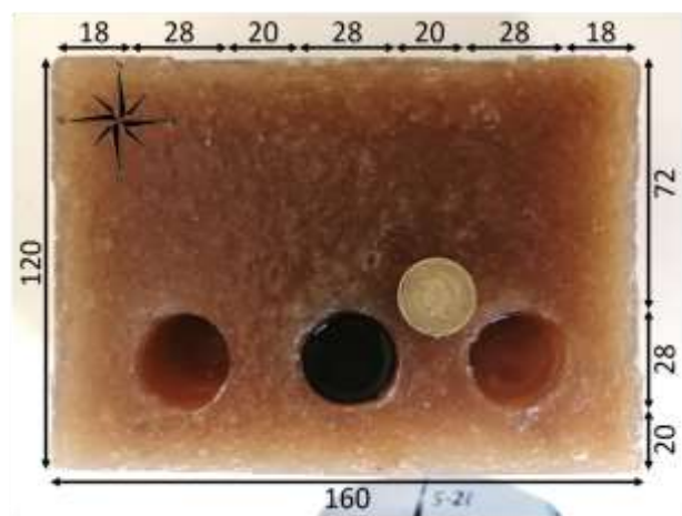
Fig. 1 Top view of the tissue-mimicking phantom with three cylindrical wells. The probe is visible on the South face. A £1 coin is included for scale. Dimensions have been stated in mm.
