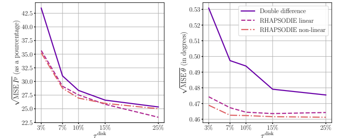
Fig. 9: Comparison of the MSE between the true map and the estimated map of the polarized intensity I^P and of the angle of polarization \theta for the Double Difference and the linear and non-linear RHAPSODIE methods with deconvolution.
