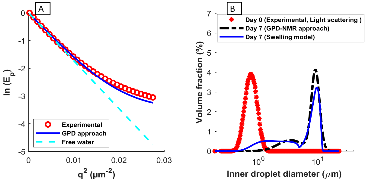
Fig. 4. A) Normalized signal attenuation in log as a function of q^2 = (\gamma g \delta)^2 . B) Size distribution of the inner droplets. The double emulsion is prepared with \phi_{inner} = 30\% and \phi_{outer} = 10\% . The fit of the GPD approach is done using eqs. 1, 2, and 4: p_{mix} = 0.96 , \sigma_1 = 0.5 , d_{50,1} = 1.6 \mu\text{m} , \sigma_2 = 0.16 , d_{50,2} = 8.4 \mu\text{m} and D_e = 1.5 \times 10^{-9} .
