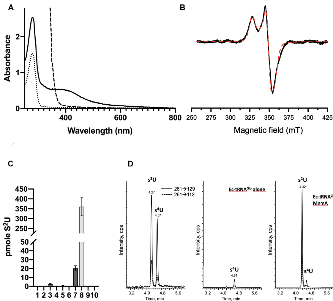
Figure 2. Spectroscopic and enzymatic characterizations of E. coli MnmA. (A) UV-visible spectra of 40 \mu M apo-MnmA (dotted line), 40 \mu M holo-MnmA (thick line) and reduced holo-MnmA after 20 min of incubation with 1 mM dithionite (dashed line). The spectra were recorded with 40 \mu M protein in 50 mM Tris-HCl (pH 7.5), 200 mM NaCl, 5 mM DTT in 1 cm (apo-MnmA and reduced holo-MnmA) or 1 mm (holo-MnmA) pathlength cuvettes and normalized. (B) X-band EPR spectrum (10 mW microwave power; modulation amplitude of 0.4 mT) of 220 \mu M holo-MnmA reduced with 5.5 mM dithionite at 15 K. The experimental (black solid line) and simulated (dashed line) spectra are superimposed. The cluster was simulated with the following values of the g-tensor: g_x = 1.880 , g_y = 1.920 , g_z = 2.045 and Gaussian distribution deviations \sigma(g_x) = 0.04 , \sigma(g_y) = 0.02 , \sigma(g_z) = 0.04 . (C) In vitro tRNA sulfuration activity tests of MnmA under anaerobic conditions. After tRNA digestion, s^2U was separated by HPLC-MS/MS and quantified using a synthetic s^2U standard. The data shown are mean values based on three different experiments, with the standard error of the mean indicated as a bar. In vitro transcribed Ec-tRNA Glu (15 \mu M) was incubated for 1 h at 37°C in 50 mM Tris (pH 7.5), 200 mM NaCl with apo or holo-MnmA (wild-type or mutant) in the presence or absence of 1 mM Na 2 S, 2.5 mM MgCl 2 , 0.25 mM ATP. Ec-tRNA Glu alone 15 \mu M (1), apo-MnmA 1 \mu M (2) or 10 \mu M (3), 1 \mu M holo-MnmA and no Na 2 S (4), no MgCl 2 (5) or no ATP (6), holo-MnmA 1 \mu M (7) or 10 \mu M (8), 1 \mu M holo-MnmA D99A-C102A-C199A mutant (9) or 1 \mu M holo-MnmA D99A-C102A-C199A mutant (10). (D) HPLC MS/MS detection of s^2U and s^4U ( m/z 261). Samples were analyzed using the two transitions 261 \rightarrow 129 and 261 \rightarrow 112; the most intense one corresponds to the loss of the ribose moiety. Left: mixture of s^2U and s^4U synthetic standards (0.5 pmole injected); middle: Ec-tRNA Glu alone after hydrolysis; right: Ec-tRNA Glu (15 \mu M) after incubation with holo-MnmA (10 \mu M) in the presence of Na 2 S, ATP, MgCl 2 and hydrolysis.
