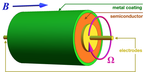
FIG. 3. The rotational diode.
