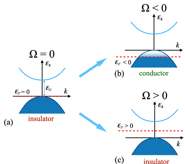
FIG. 2. The effect of rotation on the band filling of a semiconductor rotating with the angular velocity \Omega = \Omega \mathbf{e}_z in the background of magnetic field \mathbf{B} = B\mathbf{e}_z with B > 0 .
