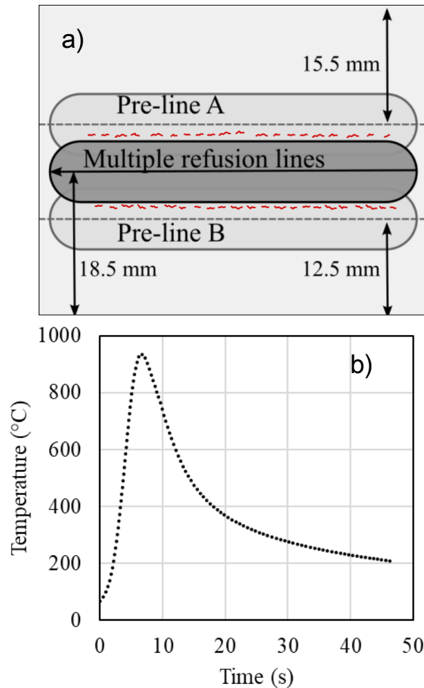
Figure 1. a) Principle of Refusion Cracking Test. Small red lines represent cracks. The length and width of pre-lines and refusion lines are 45 mm and 8 mm respectively. b) Typical temperature cycle measured during a RCT pass using a thermocouple located in the cracking region.
