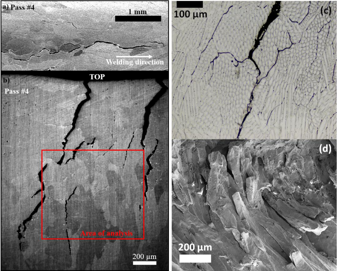
Figure 3. Observations of Base+S sample after four RCT passes. a) SEM surface observation, b) SEM cross-section observation, c) optical cross-section observation, d) SEM observation of the fracture surface of a crack.
