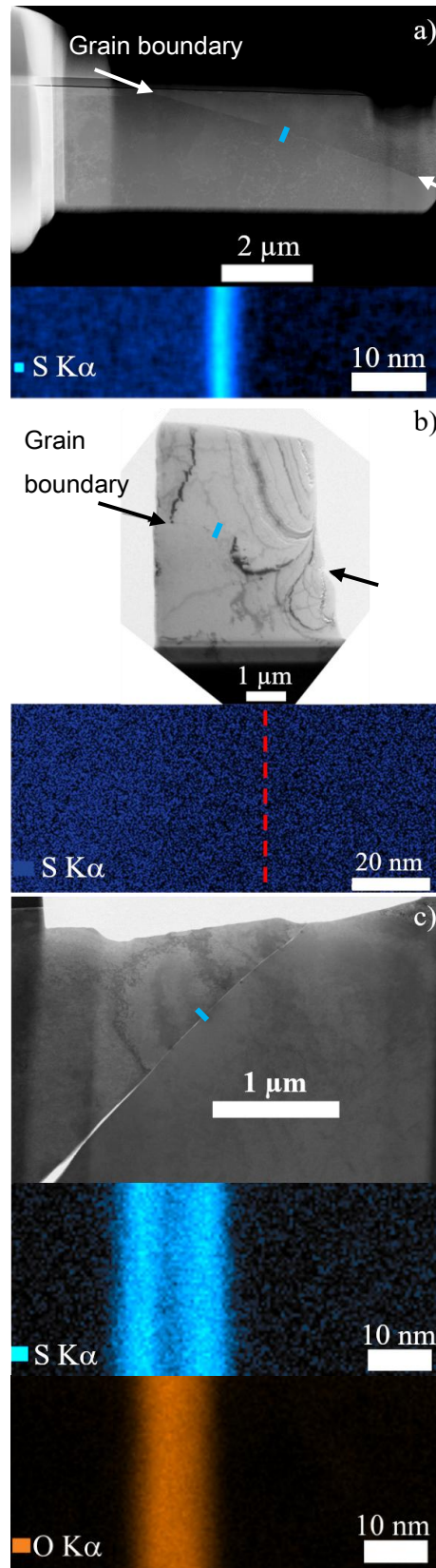
Figure 5. STEM-EDS mapping on GBs. a) control specimen, b) uncracked GB and c) cracked GB in Base+S RCT specimen. The dashed red line indicates the GB location. Blue rectangles in images indicate the mapped areas. The images were obtained using STEM high-angle annular dark field for a) and bright field TEM for b) and c).
