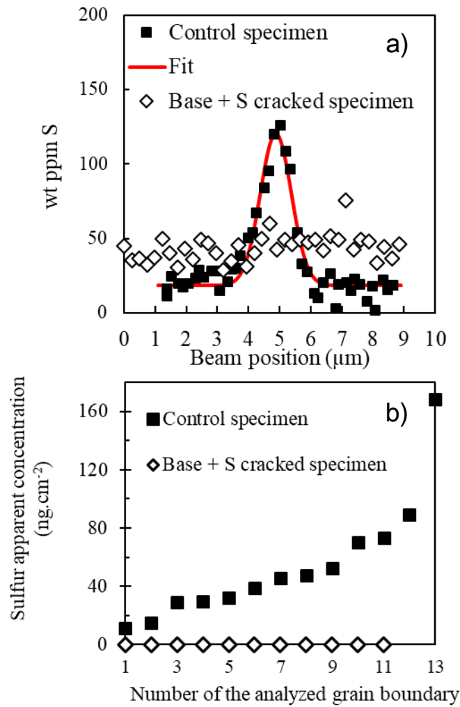
Figure 4. a) Examples of GB sulphur line scans obtained using the WDS methodology in the Base+S specimen (after four RCT passes) and in the control specimen. b) Sulphur GB concentration estimated in thirteen GBs of the control specimen and eleven GBs of the Base+S RCT specimen.
