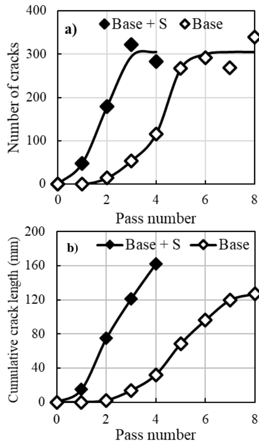
Figure 2. RCT results for Base and Base+S alloys. a) Number of cracks. b) Cumulative crack length.
