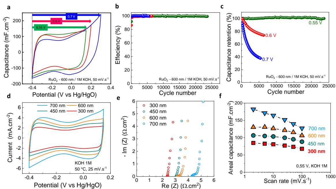
Fig. 3 | Electrochemical properties of the hRuO 2 films in 1M KOH. a. CV plots of the hRuO 2 films (400 electrodeposition cycles / 600 nm) between -0.4 and 0.15, 0.2 and 0.3 V vs Hg/HgO at 50 mV.s -1 . b-c. Evolution of the coulombic efficiency and the capacitance retention for hRuO 2 films (400 electrodeposition cycles / 600 nm) vs the cycle number at 50 mV.s -1 and the proposed electrochemical windows. d. CV plots of the hRuO 2 films with different thickness between -0.4 and 0.15 V vs Hg/HgO at 25 mV.s -1 . e. Electrochemical Impedance Spectroscopy measured in 1M KOH for RuO 2 films with various thicknesses. f. Evolution of the areal capacitance values versus sweep rate and film thicknesses.
