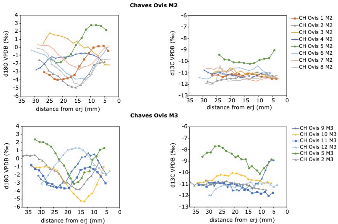
Fig 2 Results from the sequential stable carbon and oxygen isotope analysis in second and third molar ( M_2 and M_3 ) enamel bioapatite. Each sample is located in the tooth crown relative to its distance from the enamel-root junction (ERJ)
