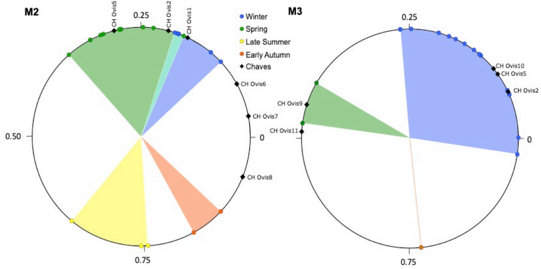
Fig. 3: Distribution of sheep births at Chaves, as reflected by the position of the maximum \delta^{18}O value in tooth crown (x0) normalized to the period of the cycle (X). The birth season is compared with modern reference sheep (Carneiane CAR: Blaise and Balasse, 2011; Rousay ROU: Balasse et al., 2012a, 2017). Blue, green, yellow and orange color areas represent normalized range values obtained from modern specimens (colored dots).
