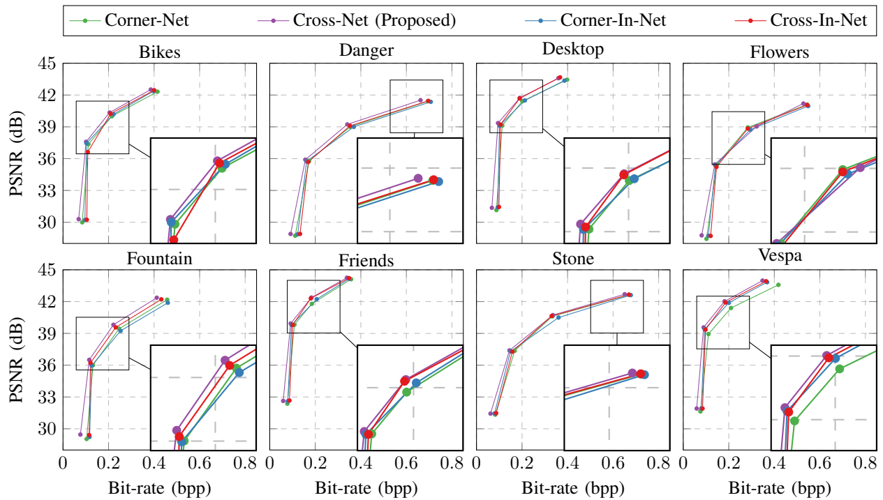
Fig. 5: RD performance comparison between four different variations of the proposed DLFC scheme based on the arrangements of the reference views shown in Fig. 2 (b-e), at quantization indices M = [1, 4, 7, 8] , using PSNR as distortion metric.
