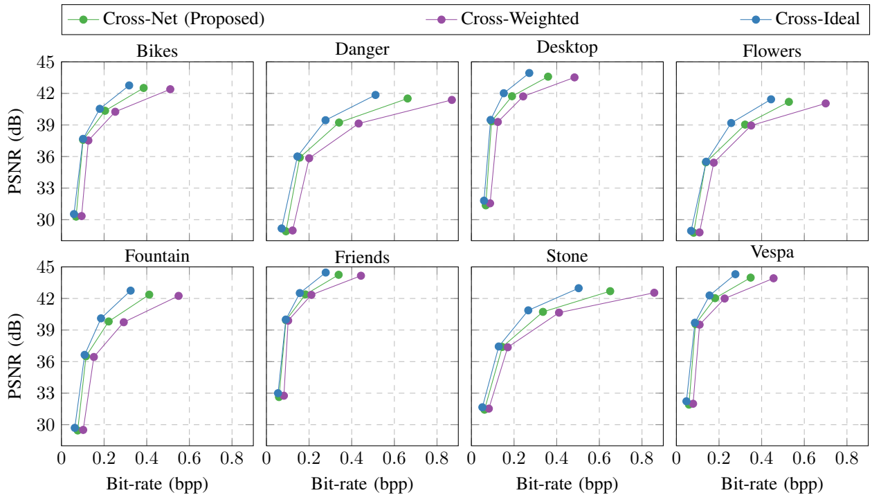
Fig. 6: RD performance comparison between different variations of the proposed DLFC scheme utilizing three different residual estimation methods, at quantization indices M = [1, 4, 7, 8] , using PSNR as distortion metric.
