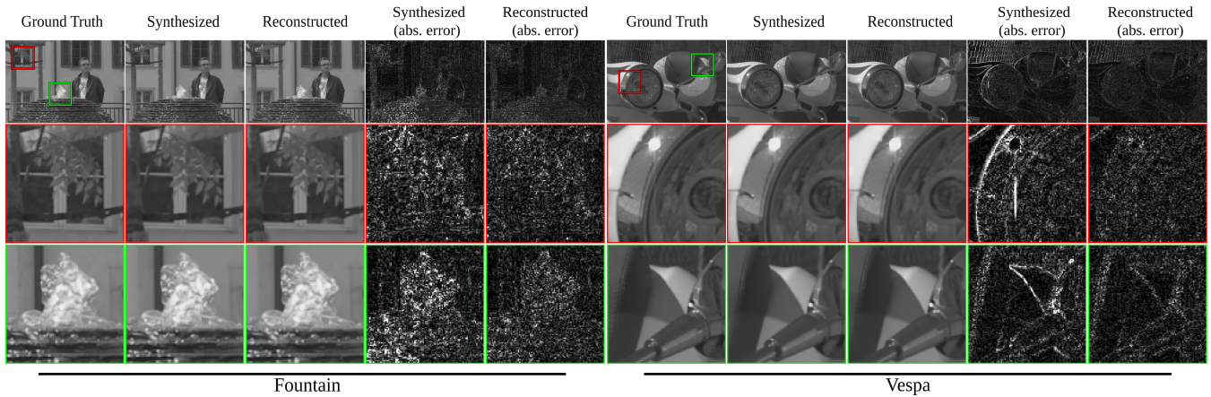
Fig. 8: Visual comparison between the outputs of stages in the proposed decoding scheme to decode the central view of the two LF sequences i.e. Fountain and Vespa at quantization index M = 8 . The ground truth image and its corresponding zoomed patches are shown on the left. The synthesized and the reconstructed WZ view along with the corresponding absolute errors (range normalized to 0.00 – 0.04) are shown in the next four columns. The zoomed patches are extracted from the highlighted regions in the ground truth images.
