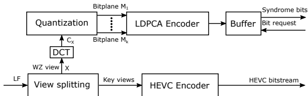
Fig. 1: Block diagram of transform-domain Wyner-Ziv encoder.
