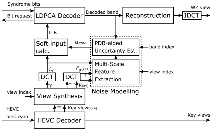
Fig. 3: Block diagram of transform-domain Wyner-Ziv decoder.
