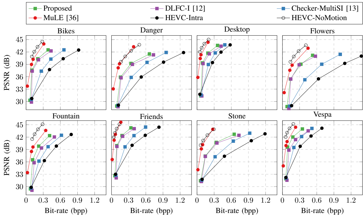
Fig. 7: RD performance comparison of distributed source coding and conventional coding schemes using PSNR as distortion metric at quantization indices M = [1, 4, 7, 8] , whereas, the quantization parameters specified in Table VII are used for both HEVC plots.
