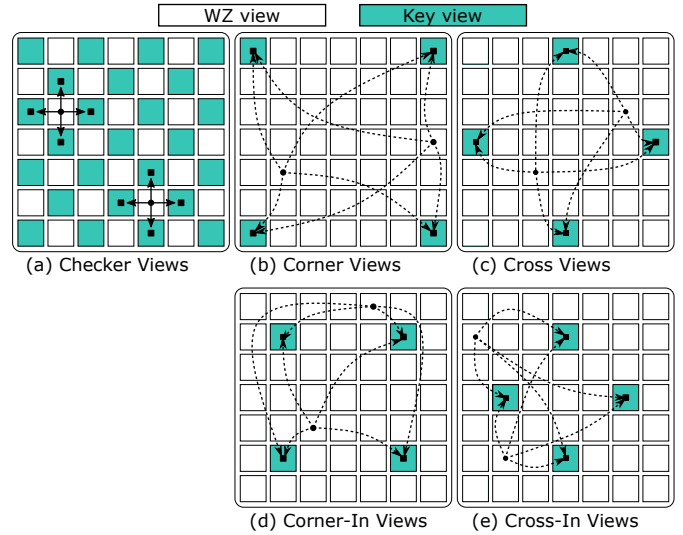
Fig. 2: View splitting modes.
