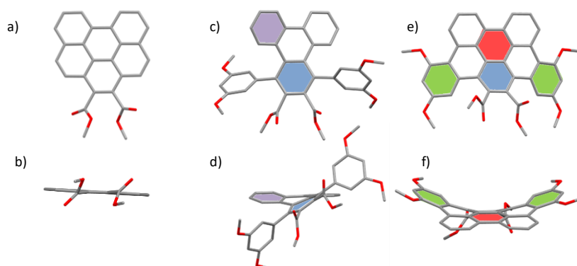
Figure 3. Crystallographic structure of 211 (top (a) and side view (b)) 6 (top (c) and side view (d)) and 8 (top (e) and side view (f)).
