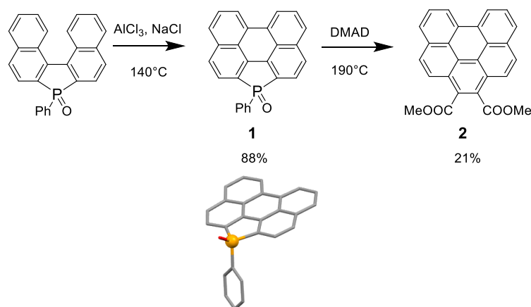
Scheme 1. Synthesis of 2 and crystallographic structure of 1
