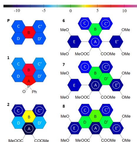
Figure 2. Visualization of the NICS(0) values (B3LYP/6-311+G**/B3LYP/6-31+G*) of compounds P , 1 , 2 and 6-8 . The NICS(0) values (which can be defined unambiguously also in the curved molecules) were presented, nevertheless the NICS(1) values show the same tendencies, see Table S18.
