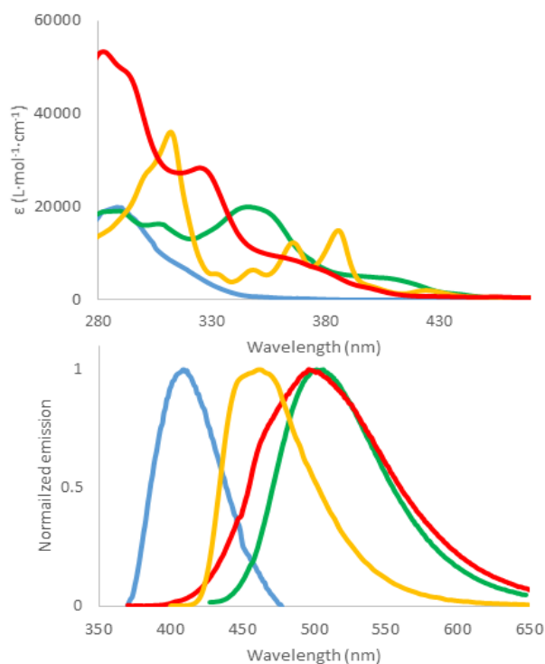
Figure 4. UV-vis absorption (top) and emission (down) of 2 (yellow), 6 (blue), 7 (red) and 8 (green) in diluted DCM. (all compound are excited at \lambda_{max} except 2 ( \lambda_{exc} = 386 nm))
