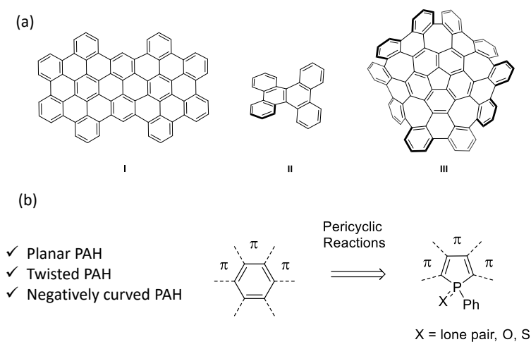
Figure 1. (a) Representative examples of planar ( I ), twisted ( II ) and negatively curved PAHs ( III ). (b) Synthetic strategy devised in this article.
