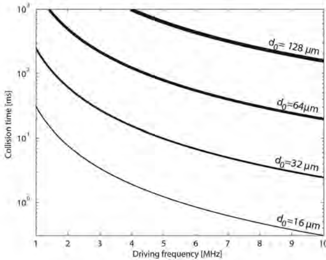
Figure 9 – Collision times of individual encapsulated microbubbles as a function of driving frequency at given distances d_0 , using p_a = 20 kPa, R_0 = 1.25 \mu\text{m} , \kappa = 5 \times 10^{-6} \text{ m}^2 \text{ N}^{-1} and \rho = 998 \text{ kg m}^{-3} .
