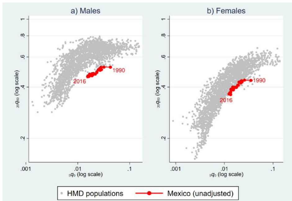
Figure 12: Child mortality ( sq_0 ) by old age mortality ( 20q_{60} ) by sex, Mexico (unadjusted, 1990–2016) compared with HMD populations (post-1950)
