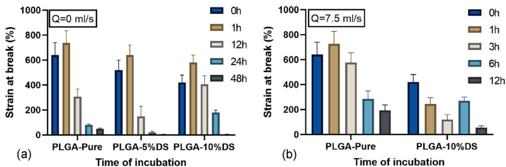
Fig. 10. Strain at break of the PLGA samples with different percentages of DS at different times of in-vitro tests under the (a) static and (b) continuous state.
