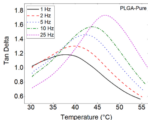
Fig. 4. Increase of glass transition temperature during multi frequency DMTA tests.
