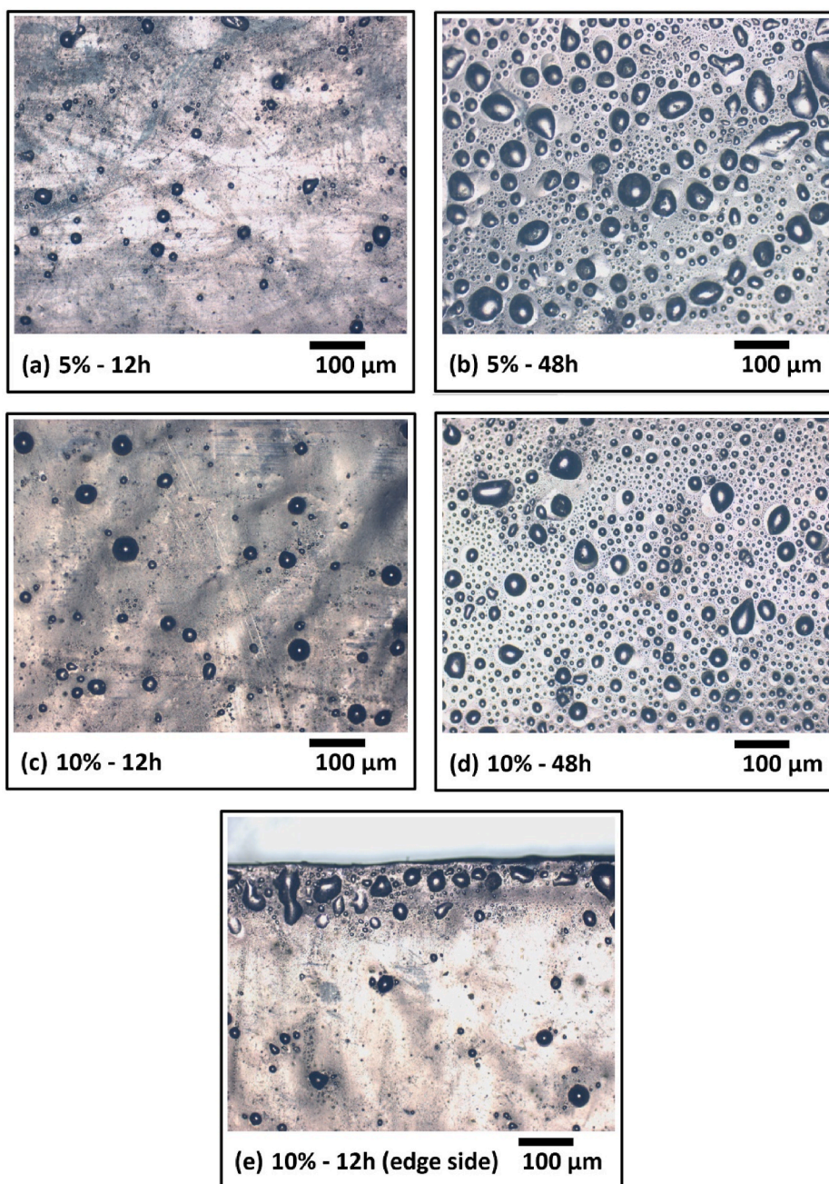
Fig. 1. Optical microscopic observations of the samples (a) PLGA-5%DS after 12 h, (b) PLGA-5%DS after 48 h, (c) PLGA-10%DS after 12 h, (d) PLGA-10%DS after 48 h, (e) PLGA-10%DS after 12 h from the edge of the sample, of drug release test under the static state.
