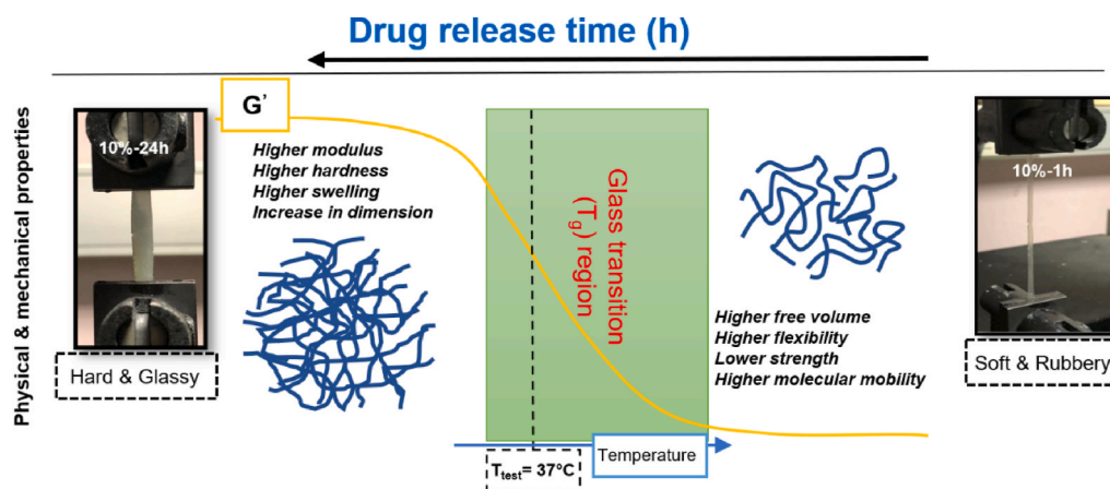
Fig. 18. Schematic of the variation of the polymer properties during and after drug release.
