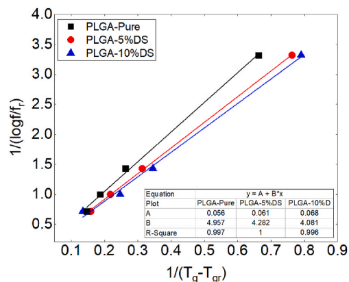
Fig. 5. Linear regression of WLF equation on the results obtained from DMA tests for the PLGA samples.
