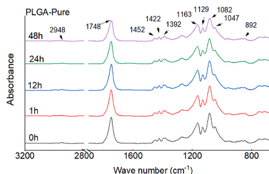
Fig. 14. FTIR spectroscopy of PLGA-Pure after certain times of incubation at the static state.
