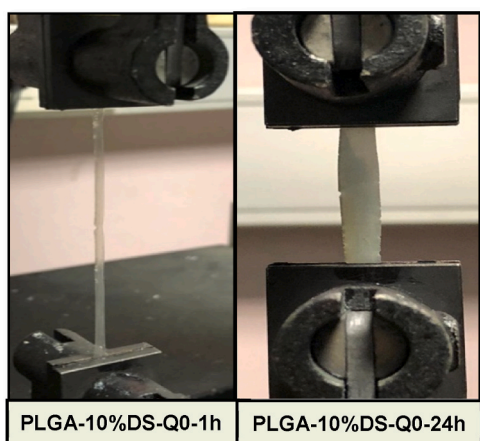
Fig. 11. Tensile test of the PLGA-10%DS after 1 h and 24 h of drug release test at static state.
