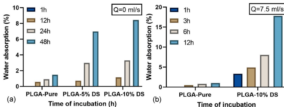
Fig. 17. Water absorption percentages for PLGA-Pure, PLGA-5%DS and PLGA-10%DS at flow rates of (a) 0 and (b) 7.5 ml/s.
