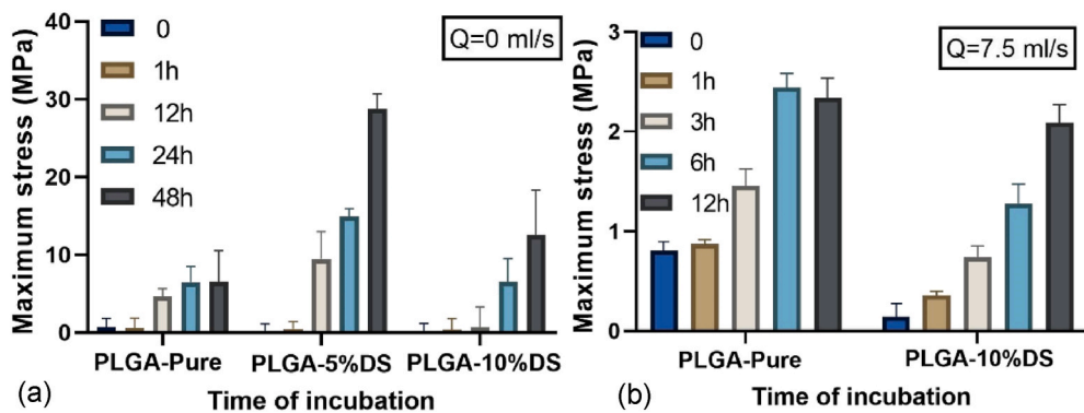
Fig. 9. Maximum stress of the PLGA samples with different percentages of DS at different times of in-vitro tests under the (a) static and (b) continuous state.
