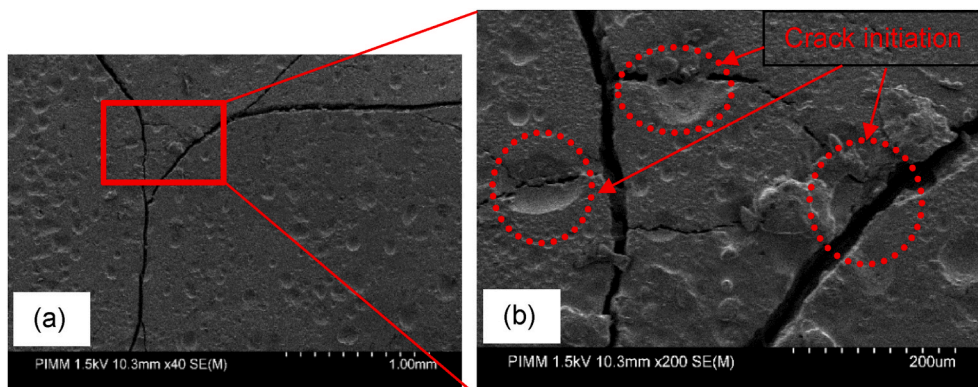
Fig. 13. SEM micrographs of the PLGA-10%DS after drug release of 48 h under the static state after tensile test with the magnification of (a) 1 mm and (b) 200 μm.
