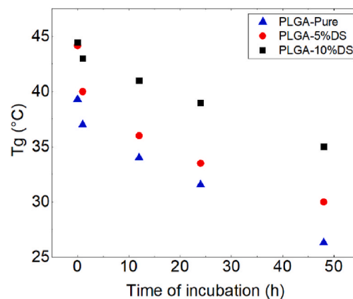
Fig. 3. Evolution of the glass transition temperature ( T_g ) of PLGA-Pure, PLGA-5%DS and PLGA-10%DS according to the test time at the static state.
