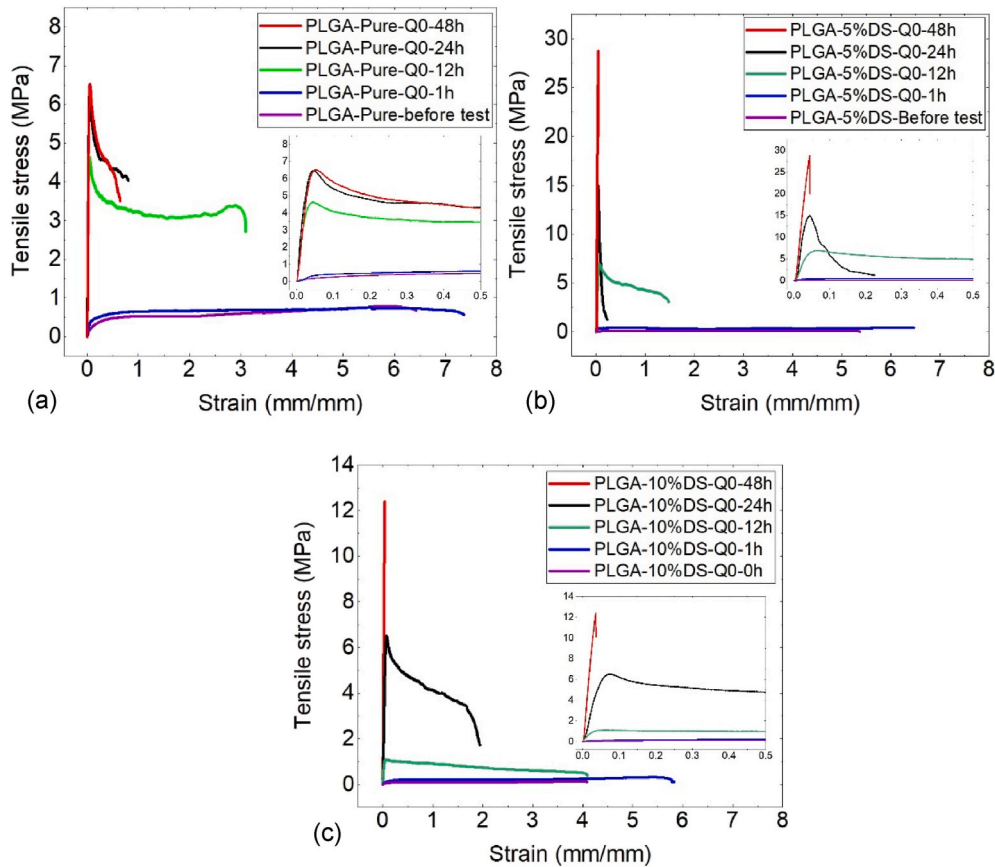
Fig. 6. Stress-strain curves of the PLGA-pure, PLGA-5%DS, and PLGA-10%DS after static test.
