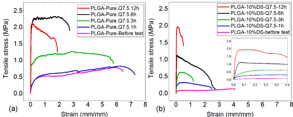
Fig. 7. Stress-strain curves of (a) PLGA-Pure and (b) PLGA-10%DS after in-vitro test under the flow rate of 7.5 ml/s.
