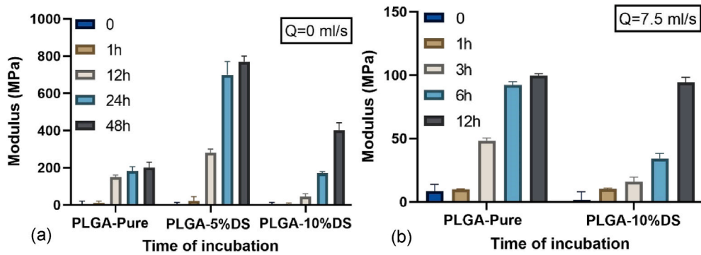
Fig. 8. Young's modulus of the PLGA samples with different percentages of DS at different times of in-vitro tests under the (a) static and (b) continuous state.
