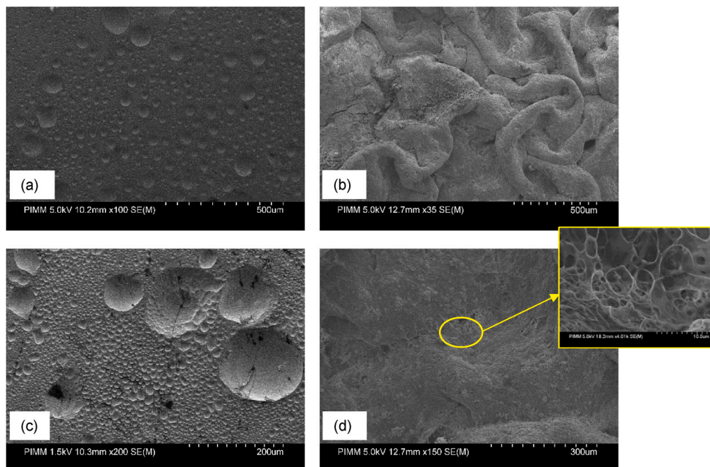
Fig. 2. SEM micrographs of PLGA-10%DS after 48 h of drug release at (a), and (c) the flow rate of 0, (b), and (d) flow rate of 7.5 ml/s, but at different magnifications.
