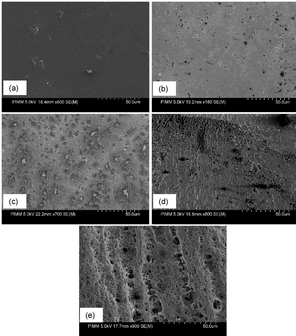
Fig. 15. SEM micrographs of the PLGA-Pure samples in PBS at zero flow rate after (a) 0, (b) 1, (c) 12, (d) 24, (e) 48 h.
