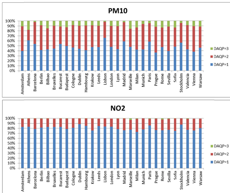
Fig. 8 relative potential apportionment between D_{AQP} = 1 (blue), D_{AQP} = 2 (red), and D_{AQP} = 3 (green), for PM_{10} (top) and NO_2 (bottom)
