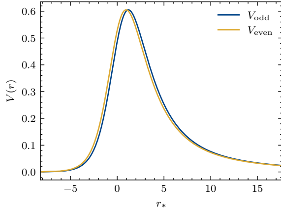
FIG. 1 Illustration of the effective potentials (for axial and polar modes) for a Schwarzschild black hole. The parameters are such that r_s = 2 (i.e. the mass of the black is 1 in natural units) and \ell = 2 here.
