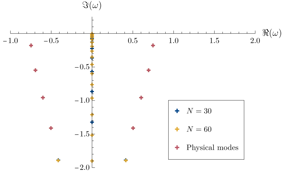
FIG. 2 Quasinormal modes numerically found by Mathematica for r_s = 1 and \ell = 2 ( \lambda = 2 ). The blue dots are generalised eigenvalues for N = 30 , the orange dots generalised eigenvalues for N = 60 , and the red dots are the modes detected (eigenvalues that change by a factor 10^{-3} or less). All the dots present on the imaginary axis correspond to spurious modes. We observe a symmetry with respect to the imaginary axis. The positions of the first modes are \omega_0 = \pm 0.747 - 0.178i , \omega_1 = \pm 0.693 - 0.548i and \omega_2 = \pm 0.602 - 0.957i .
