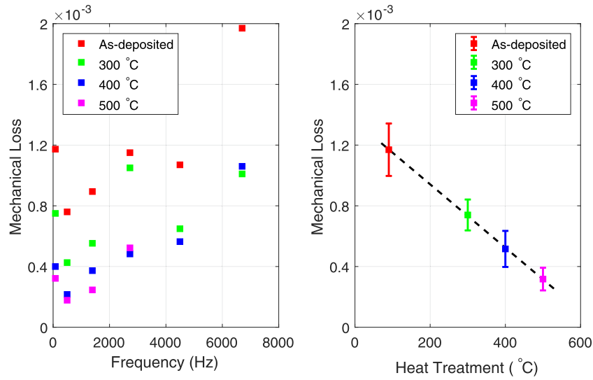
Figure 13. Coating loss of IBS \text{Ta}_2\text{O}_5\text{-ZrO}_2 thin film MLD2018, as measured on a clamped \sim 100 \mu\text{m} thick fused-silica cantilever at ambient temperature. Left: (a) the loss was measured as a function of frequency on the as-deposited sample, then re-measured after progressive annealings at 300, 400 and 500 °C; right: (b) frequency-averaged coating loss \bar{\varphi} as a function of annealing temperature. The coating loss decreased after each annealing treatment.
