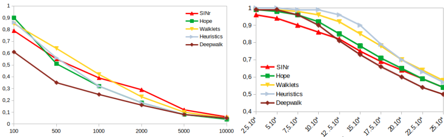
Fig. 4. precision@k , the proportion among the k most probable pairs that are edges according to the classifier trained on link prediction on Cts (at left) and Fb (at right).
