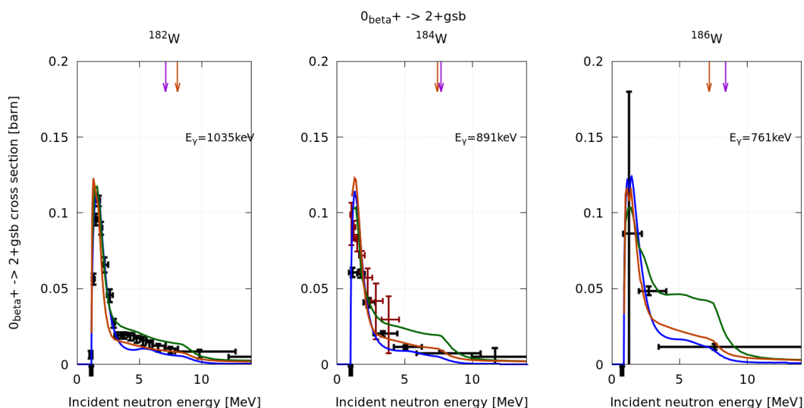
Figure 4. Same as figure 1, for the 0^+ beta to 2^+ gsb transition. Data could be extracted from the ^{\text{nat}}\text{W} dataset only for ^{184}\text{W} .
