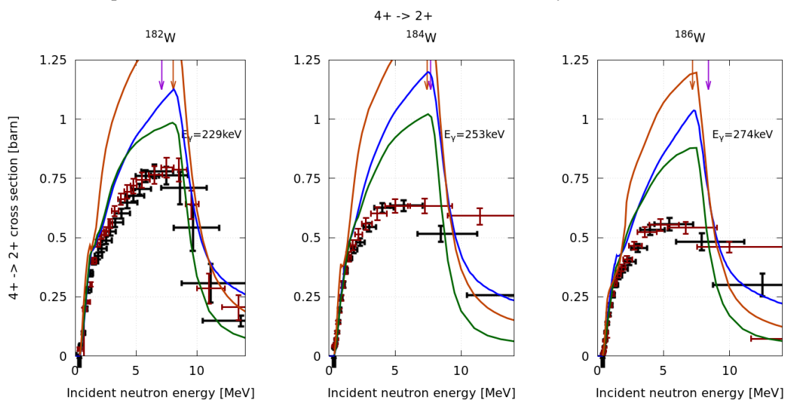
Figure 2. Same as figure 1, for the 4^+ to 2^+ transition in the ground state band.
