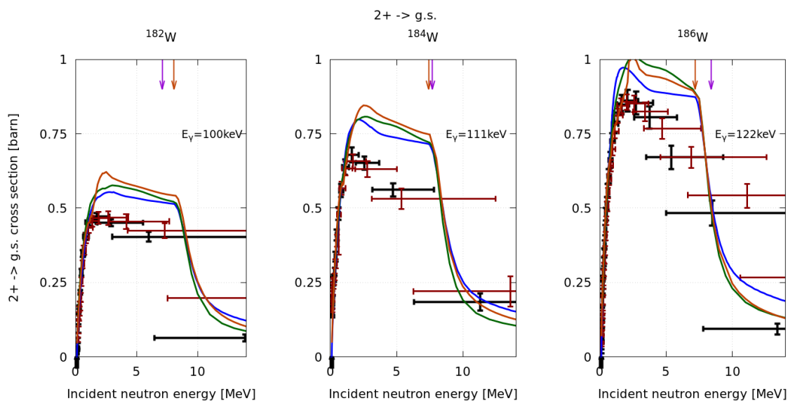
Figure 1. (n, n' \gamma) cross sections measured with GRAPhEME for the isotopes ^{182}\text{W} (left), ^{184}\text{W} (center), ^{186}\text{W} (right), for the first excited state ( 2_{\text{gsb}}^+ ) to the ground state transition. The data from isotopic targets are represented with black crosses, the data from the ^{\text{nat}}\text{W} target in red (corrected for ^{183}\text{W}(n, 2n \gamma) contamination for ^{182}\text{W} ). It is compared to TALYS-1.73 (blue line), EMPIRE (orange line) and CoH3 (green line) calculations. The excitation energy of the decaying level is marked with the black up-pointing arrow on the bottom axis. The neutron separation energy S_n and proton separation energy S_p are marked with the orange and purple down-pointing arrows at the top, respectively.
