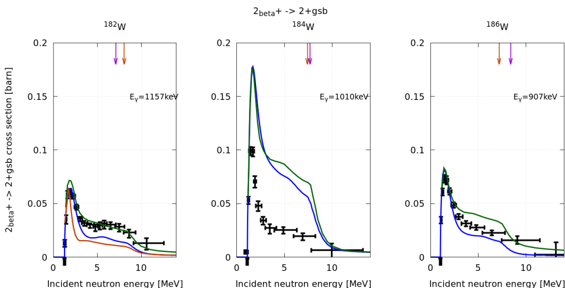
Figure 6. Same as figure 1, for the 2^+_{\text{beta}} to 2^+_{\text{gsb}} transition. No data could be extracted from the ^{\text{nat}}\text{W} dataset.
