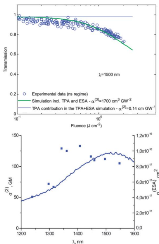
Figure 64. Top: OPL performances of compound 170 (0.1 M in CH 2 Cl 2 , \lambda_{ex} = 1500 nm, 7 ns pulses, 10 Hz). Bottom: comparison between 2PA (squares) and ESA (line) in the NIR range. Reproduced from reference 356 with permission from the PCCP Owner Societies.
