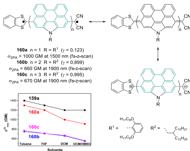
Figure 51. Push-pull perylene-based diradicaloids and plot of the solvent-dependent 2PA cross-section maxima of the series 160 . Adapted with permission from reference 333 . Copyright 2015 American Chemical Society.
