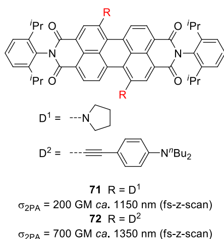
Figure 25. Perylene-bis(dicarboximides) D-A-D structures.
