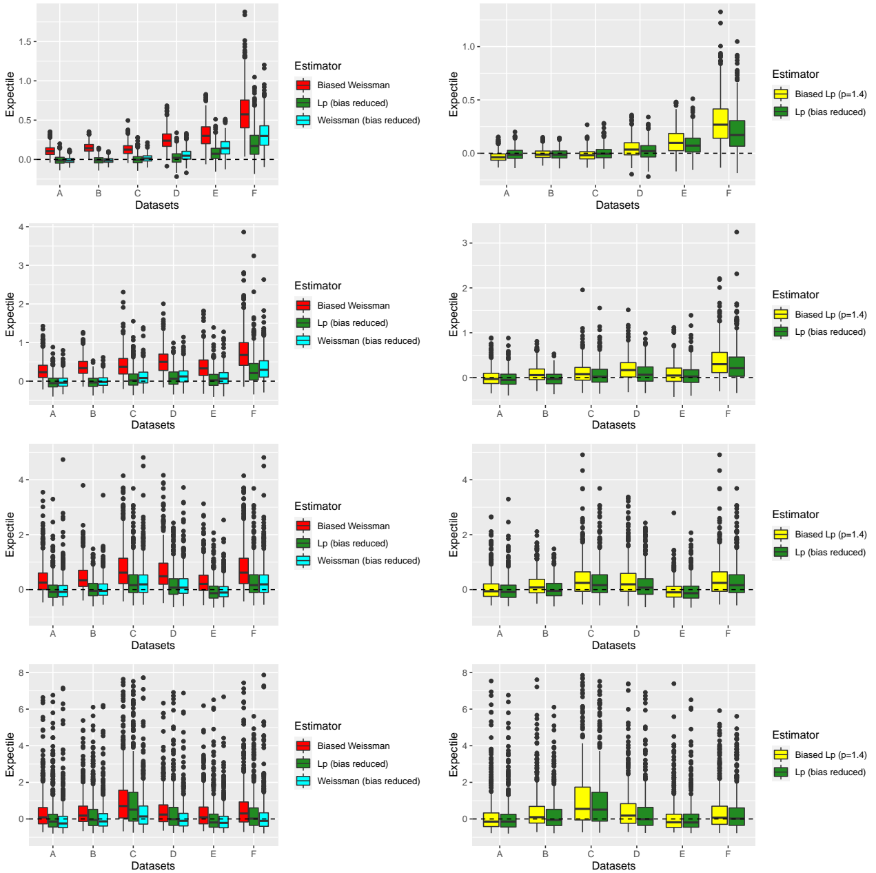
Figure 4: Extreme expectile estimation at level \alpha'_n = 1 - 1/n = 0.999 for n = 1,000 . Left panels: boxplots of \hat{q}_{\alpha'_n}^*(2)/q_{\alpha'_n}(2) - 1 (red boxes), \tilde{q}_{\alpha'_n, p^*}^{*,RB}(2)/q_{\alpha'_n}(2) - 1 (green boxes) and \hat{q}_{\alpha'_n}^{*,RB}(2)/q_{\alpha'_n}(2) - 1 (blue boxes). Right panels: boxplots of \tilde{q}_{\alpha'_n, 1.4}^*(2)/q_{\alpha'_n}(2) - 1 (yellow boxes) and \tilde{q}_{\alpha'_n, p^*}^{*,RB}(2)/q_{\alpha'_n}(2) - 1 (green boxes). From top to bottom: \gamma = 0.1, 0.3, 0.5 and 0.7 . Model A is the Burr distribution with \rho = -1 , model B is the Fréchet distribution, model C is the Burr distribution with \rho = -0.5 , model D is the Inverse Gamma distribution, model E is the Student distribution and model F is the Generalized Pareto distribution.
