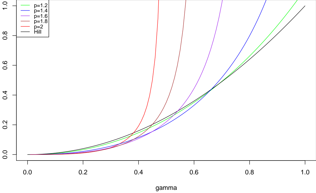
Figure 1: Asymptotic variance v_p(\gamma) for p = 1.2 (green), 1.4 (blue), 1.6 (violet), 1.8 (brown) and 2 (red), as a function of \gamma \in (0, 1) . The black curve represents v_H(\gamma) , the asymptotic variance of the Hill estimator.
