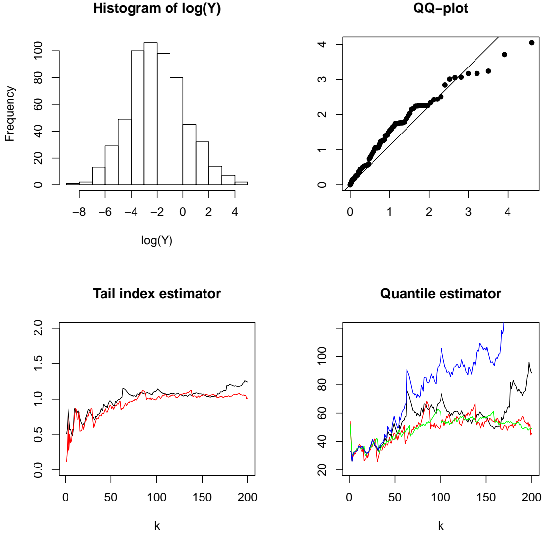
Figure 6: Tornado losses data analysis. Top left: Histogram of the log-claims. Top right: Exponential quantile-quantile plot of the log-excesses \log(Y_{n-i+1,n}/Y_{n-k,n}) (vertically) versus \log((k+1)/i) (horizontally), for 1 \leq i \leq k , with k = 100 . Bottom left: Tail index estimators \tilde{\gamma}_{1-k/n}^{(H)} (black) and \tilde{\gamma}_{1-k/n}^{(p^*)} (red) as functions of k . Bottom right: 99.5 % quantile estimators of losses (in dollars) per square yard due to tornadoes, estimated with \hat{q}_{0.995}^*(1) (blue), \hat{q}_{0.995}^{*,RB}(1) (black), \hat{q}_{0.995,1.4}^*(1) (green) and \hat{q}_{0.995,p^*}^{*,RB}(1) (red) as functions of k , where the anchor level \alpha_n is set as 1 - k/n . Throughout, p^* = 1.29 .
