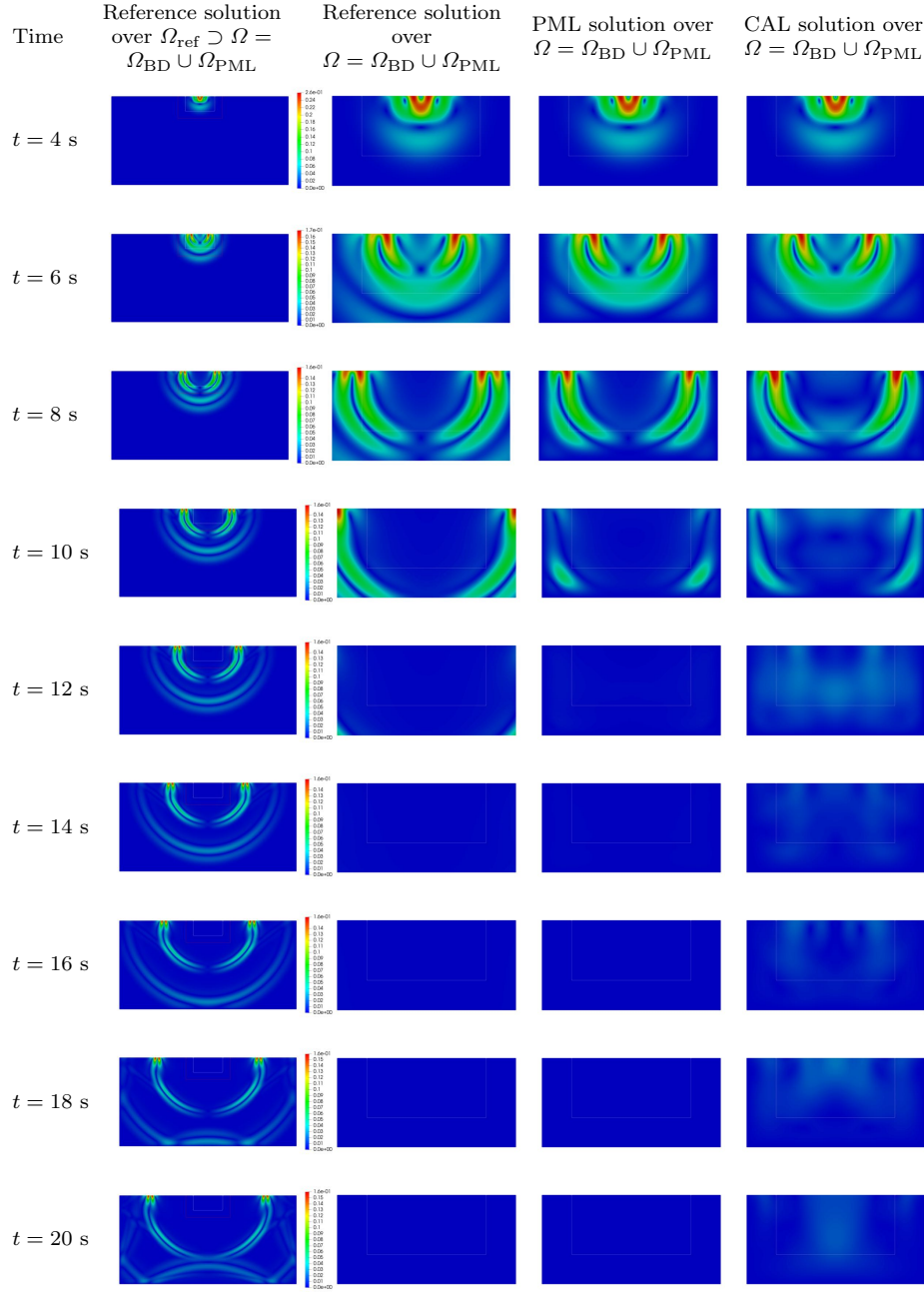
Fig. 5: Lamb's problem: snapshots of the displacement field magnitude \mathbf{x} \mapsto \|\mathbf{u}(\mathbf{x}, t)\| taken at different times t = 4, 6, 8, 10, 12, 14, 16, 18, 20 s (from top to bottom) for the reference solution over an extended computational domain \Omega_{\text{ref}} \supset \Omega = \Omega_{\text{BD}} \cup \Omega_{\text{PML}} (first column) with interface \Gamma = \partial\Omega_{\text{BD}} \cap \partial\Omega_{\text{PML}} indicated by white solid lines and the exterior boundary \Gamma_{\text{ext}} of \Omega indicated by red solid lines, the reference solution over the computational domain \Omega = \Omega_{\text{BD}} \cup \Omega_{\text{PML}} (second column), the PML solution over \Omega (third column) and the CAL solution over \Omega (fourth column)
