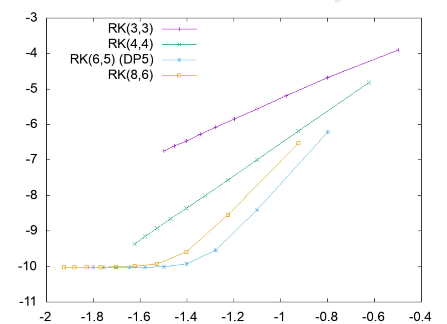
h_{(s, n)} as a function of numerical cost \frac{\Delta t}{s} in log scale
