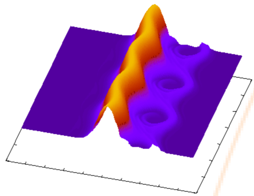
Example of filamentation process in a solution
