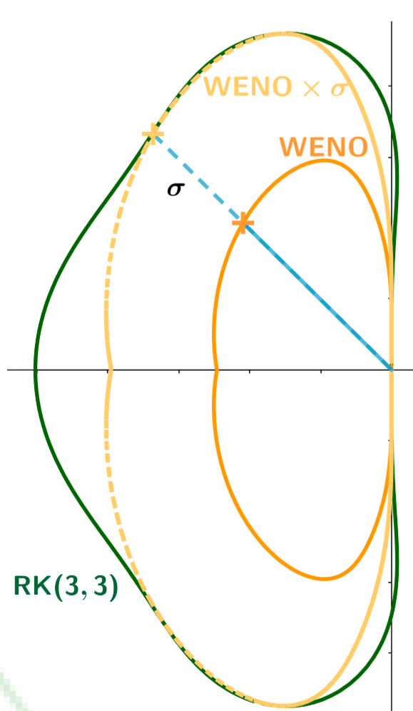
Geometric CFL interpretation
