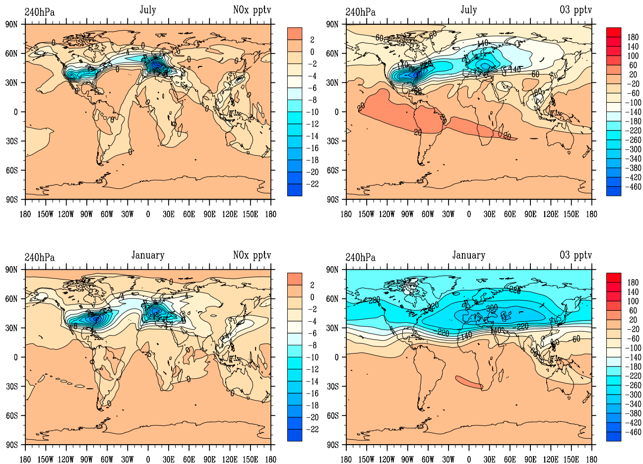
Figure 8. Distribution of the (left) \text{NO}_x and (right) \text{O}_3 variations at 240 hPa due to plume effects for experiment PL2 relative to the experiment BC. Results from the LMDz-INCA model for (top) July and (bottom) January.
