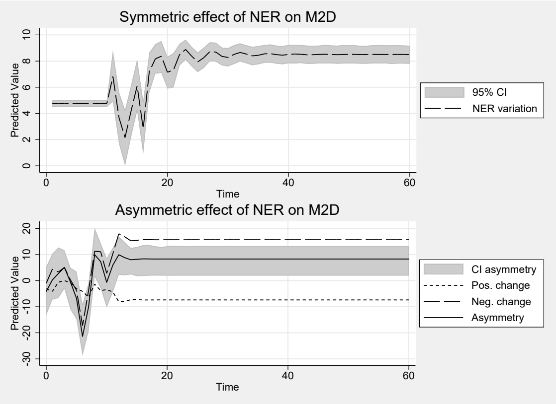
Figure 1: Dynamic multipliers
