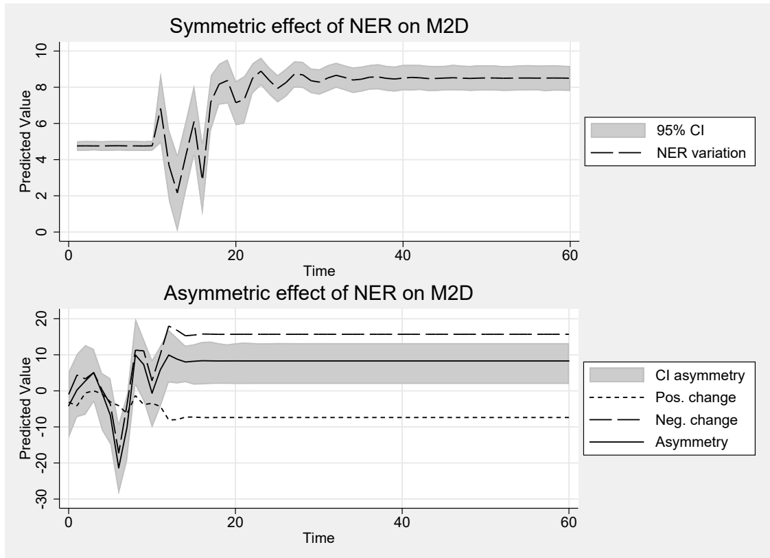
Figure 1: Dynamic multipliers
