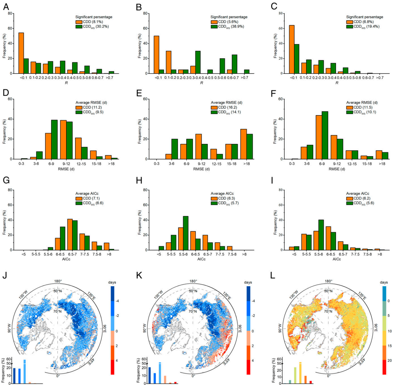
Fig. 5. Comparison between the traditional CDD model for predicting DFS and the CDD model modified to include wind speed ( CDD_{ws} ). (A, D, and G) Frequency of significant observations, RMSE (days), and the AICc using ground data, respectively. (B, E, and H) Frequency of significant observations, RMSE, and AICc using flux data, respectively. (C, F, and I) Frequency of significant observations, RMSE, and AICc for the NDVI3g data, respectively. (J and K) Differences between projected DFS using CDD and CDD_{ws} under scenarios of RCP 4.5 (J) and RCP 8.5 (K), respectively. (L) Difference between projected DFS using CDD_{ws} under the RCP 4.5 and the RCP 8.5. Significance was set at P < 0.05 .
