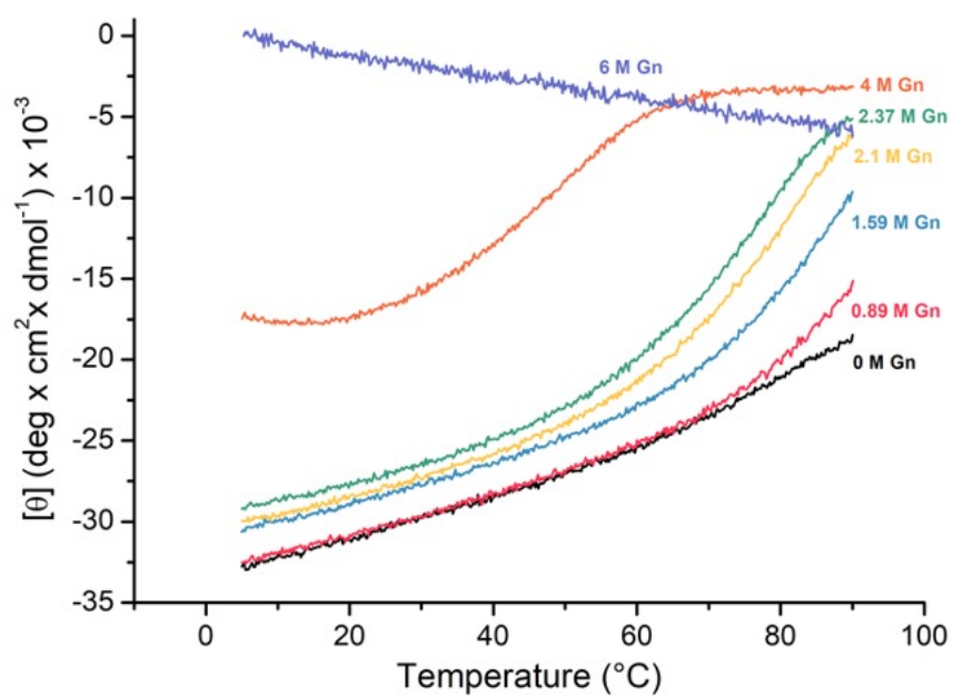
Figure S2. Melting curves measured by CD at 222 nm for the catalytic protein Het-N2 at different concentrations of guanidine hydrochloride (Gn·HCl). Thermal denaturation of Het-N2 is similar to the original DSD scaffold with dimerization constant K_D = 140 \text{ pM} . 15
