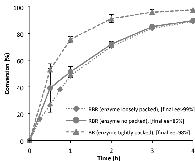
Figure 3. Synthesis of ( R )-mandelonitrile using different enzyme loadings. Conditions: Ratio benzaldehyde : HCN in acetate buffered MTBE pH 4 1:4, benzaldehyde (100 \mu L, 1 mmol), 2 ml HCN solution in acetate buffered MTBE (1.75 M) pH 4, 27.5 \mu L (0.1 mmol) 1,3,5-triisopropylbenzene as I.S. and a tea bag filled with different amounts of GtHNL -TM immobilised on 50 mg Celite R-633. The reaction was stirred at 700 rpm at 5 ^{\circ} C. Error bars correspond to duplicate (n=2).
