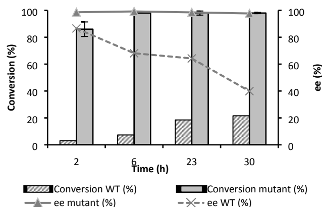
Figure 1. Synthesis of ( R )-mandelonitrile using GtHNL -WT and GtHNL -TM. Conditions: Ratio benzaldehyde : HCN in acetate buffered MTBE pH 4 1:4, 100 \mu L benzaldehyde (1 mmol), 2 mL HCN solution in acetate buffered MTBE (1.5–2 M) pH 4, 27.5 \mu L (0.1 mmol) 1,3,5-tri-isopropylbenzene as internal standard (I.S.), tea bag filled with immobilised enzyme (5 U) on 50 mg (0.1 U/mg) Celite R-633. The reaction was stirred at 1000 rpm at 5°C. Error bars correspond to duplicate (n=2).
