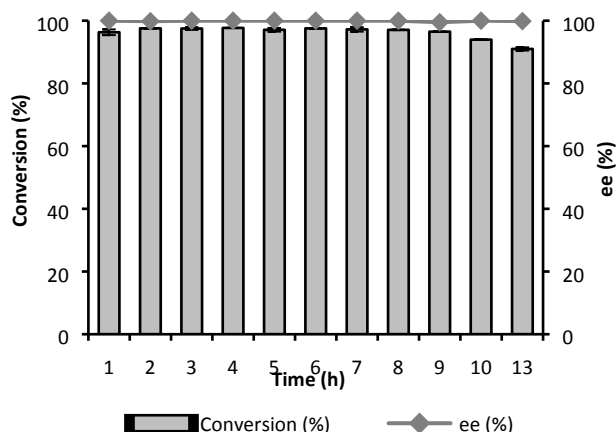
Figure 7. Stability of GtHNL-TM for the synthesis of ( R )-mandelonitrile in CFR at 0.1 mL/min. Conditions: Ratio benzaldehyde : HCN in buffered MTBE pH 4 1:4, benzaldehyde (0.5 M), HCN solution in acetate buffered MTBE (1.5-2 M) pH 4, 1,3,5 tri-isopropylbenzene (50 mM, I.S.), with GtHNL-TM immobilised on 150 mg Celite R-633 (1 U/mg = 150 U). Error bars correspond to duplicates (n=2).
