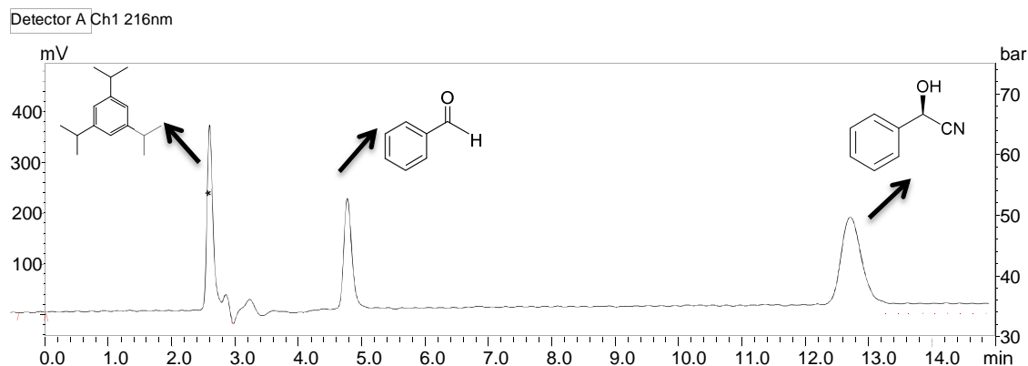
Figure S5. HPLC detection of benzaldehyde, 1,3,5 tri-isopropylbenzene and ( R )-mandelonitrile. Conditions: Ratio benzaldehyde : HCN in buffered MTBE pH 4 ~ 1:4, a CFR with GtHNL-TM immobilised on 150 mg Celite R-633 (150 U). Reactions was performed at room temperature.
