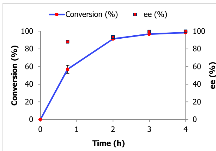
Figure S2: Kinetic trace for the synthesis of ( R )-mandelonitrile with non-immobilized GtHNL -TM. Conditions: Ratio benzaldehyde : HCN in acetate buffered MTBE pH 4 1:4, GtHNL -TM (11 mg, 50 U). The reaction was stirred at 1000 rpm at 5 °C.
